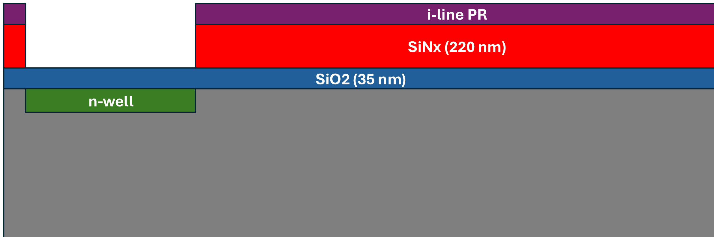
11. n-well Implantation
