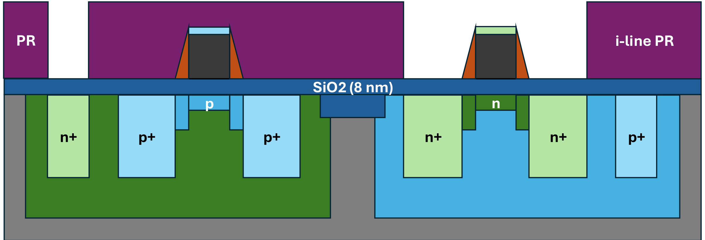
53. n+ Gate & S/D + GND Implant
