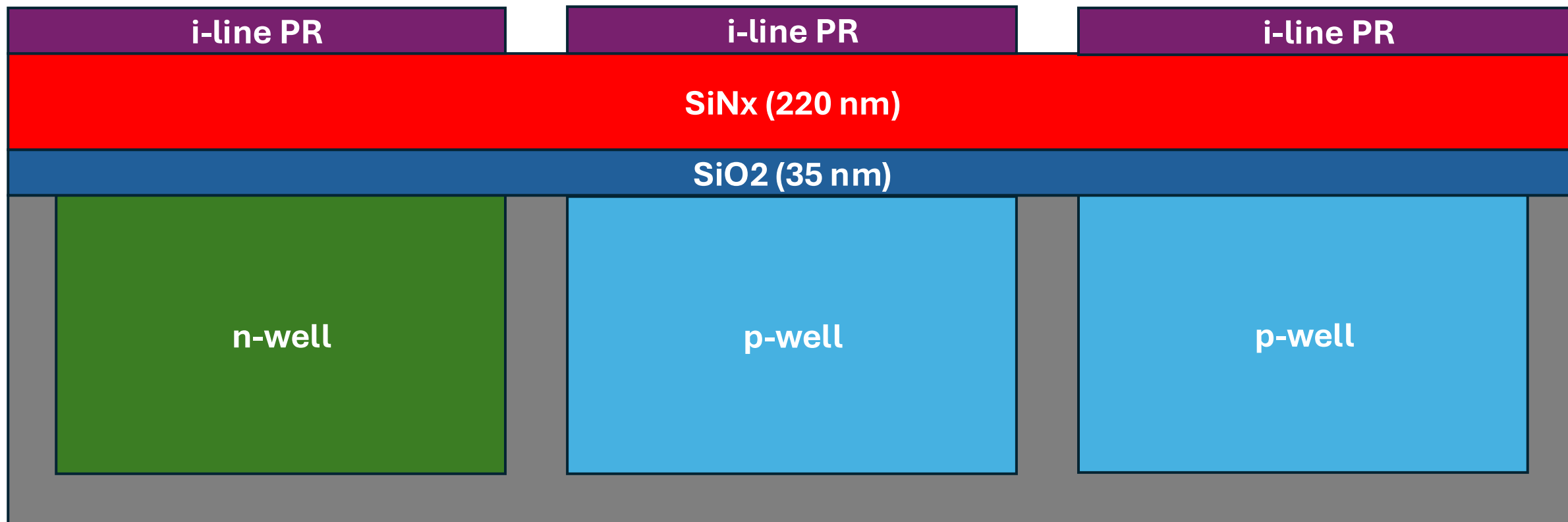
21. Active Area Litho
