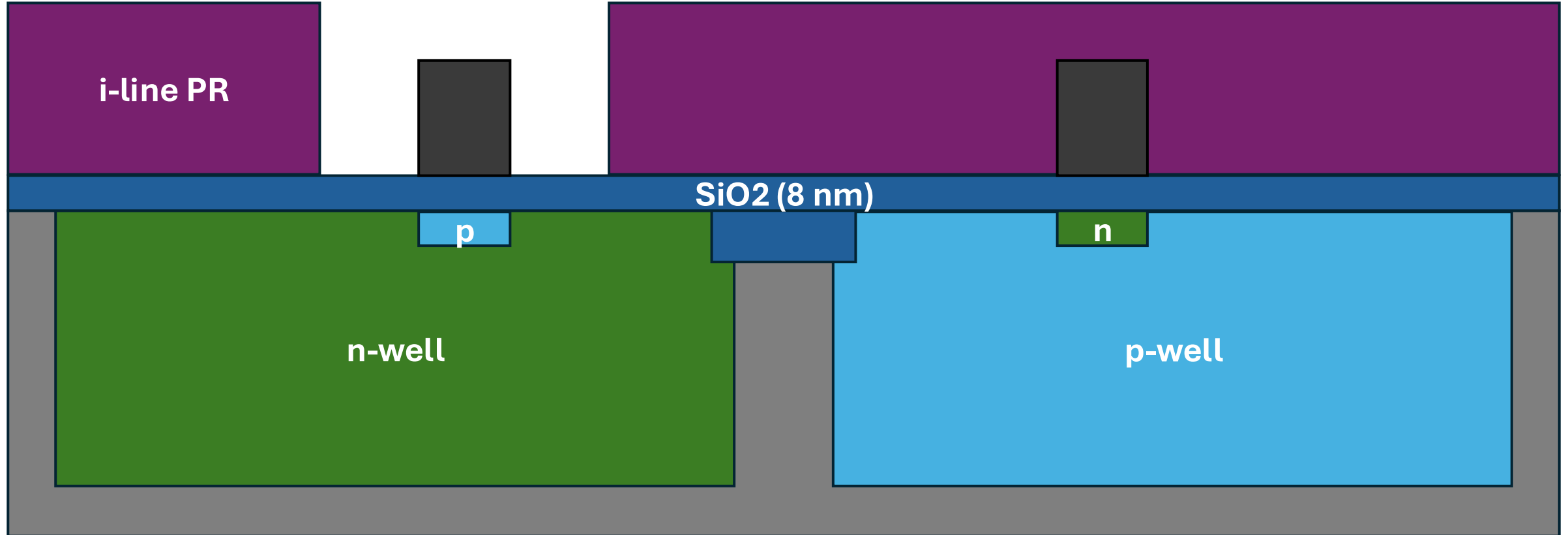
42. PMOS LDD Implant Litho
