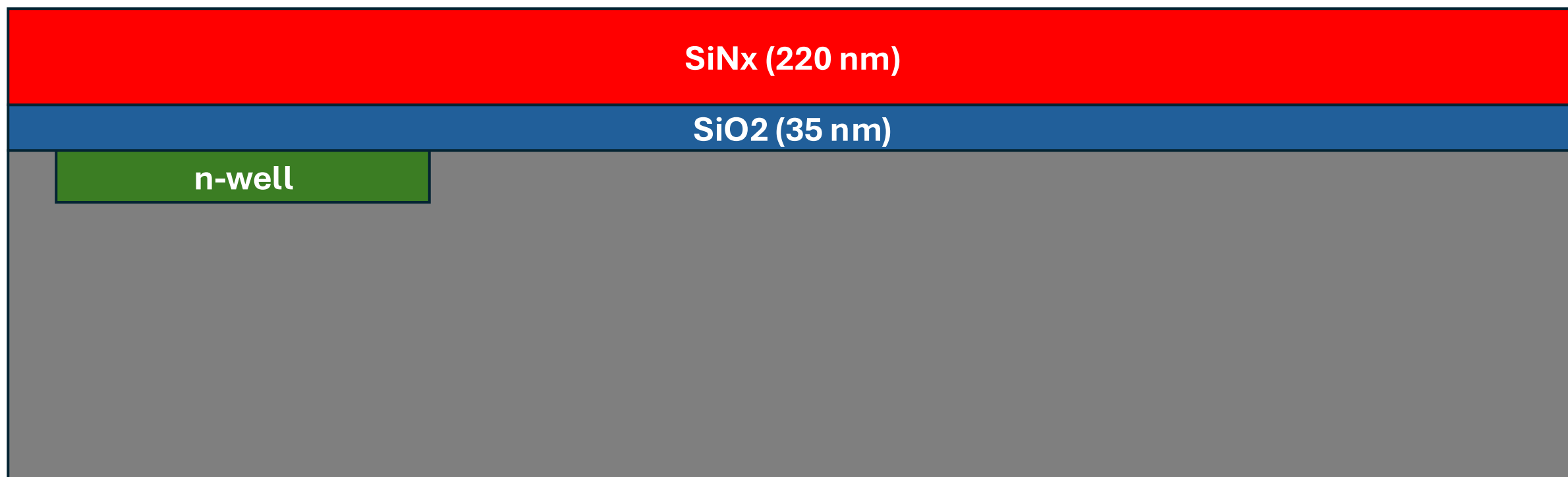
13. Pad Oxide + Nitride Deposition
