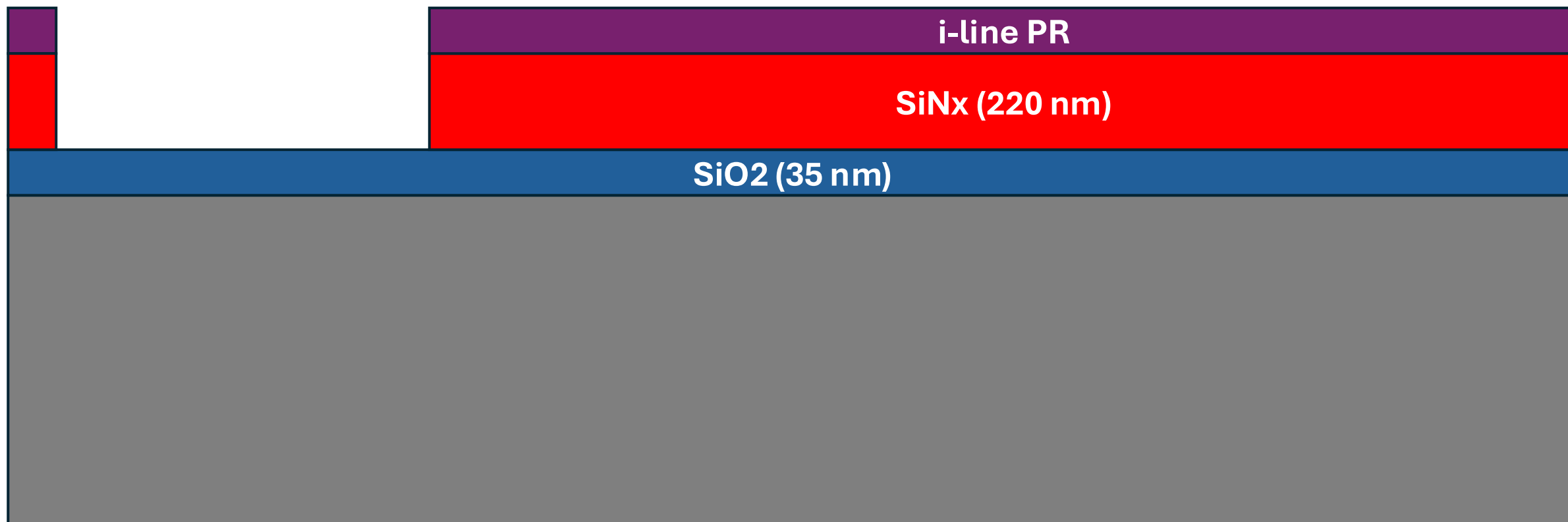
10. Nitride Wet Etch
