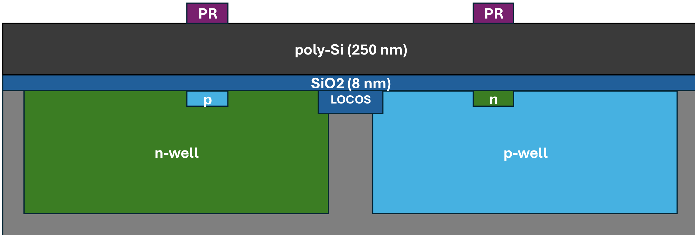
40. poly-Si Gate Litho
