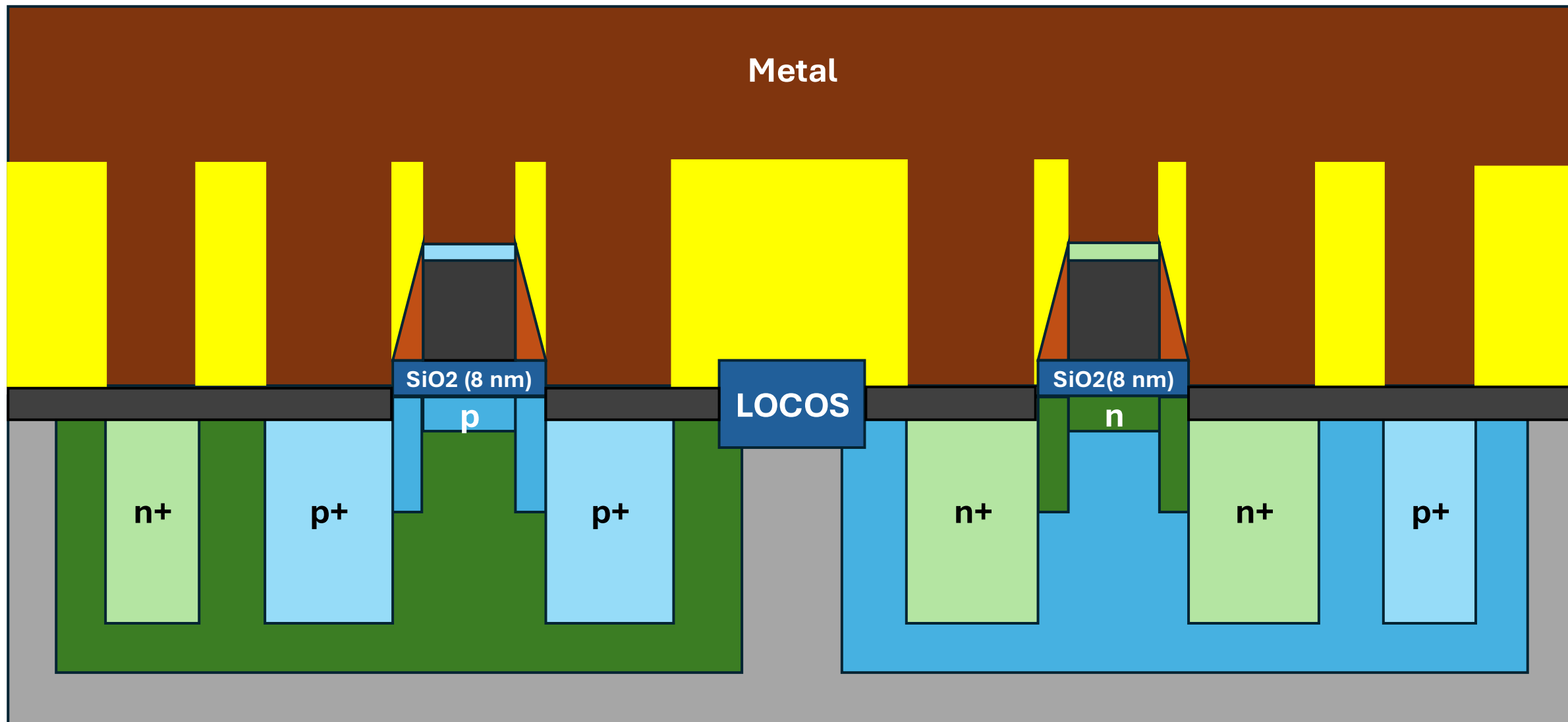
67. Metal Deposition
