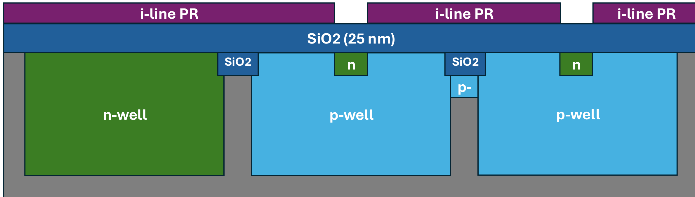
33. NMOS V t Implant
