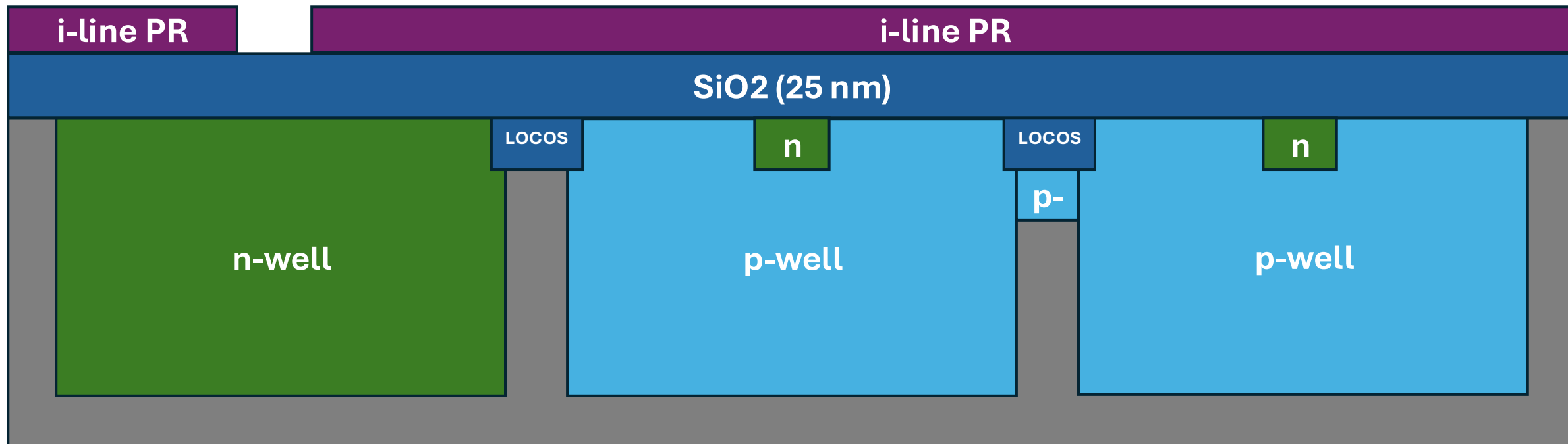
35. PMOS Vt Implant Litho
