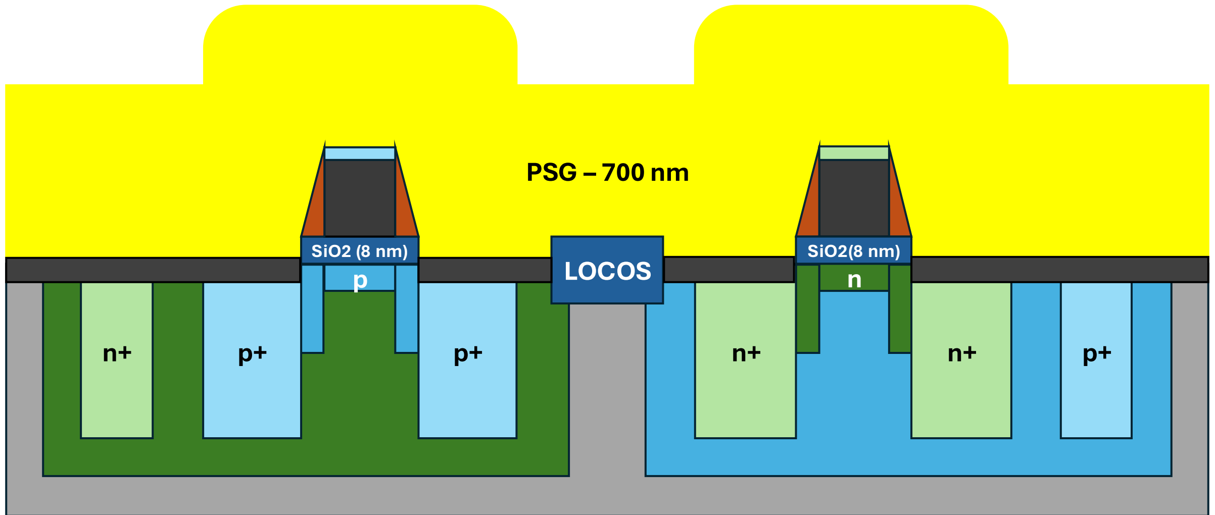
62. PSG Deposition & Densification
