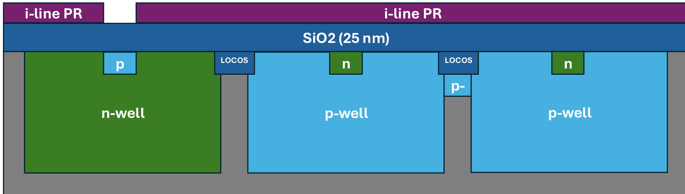
36. PMOS Vt Implant
