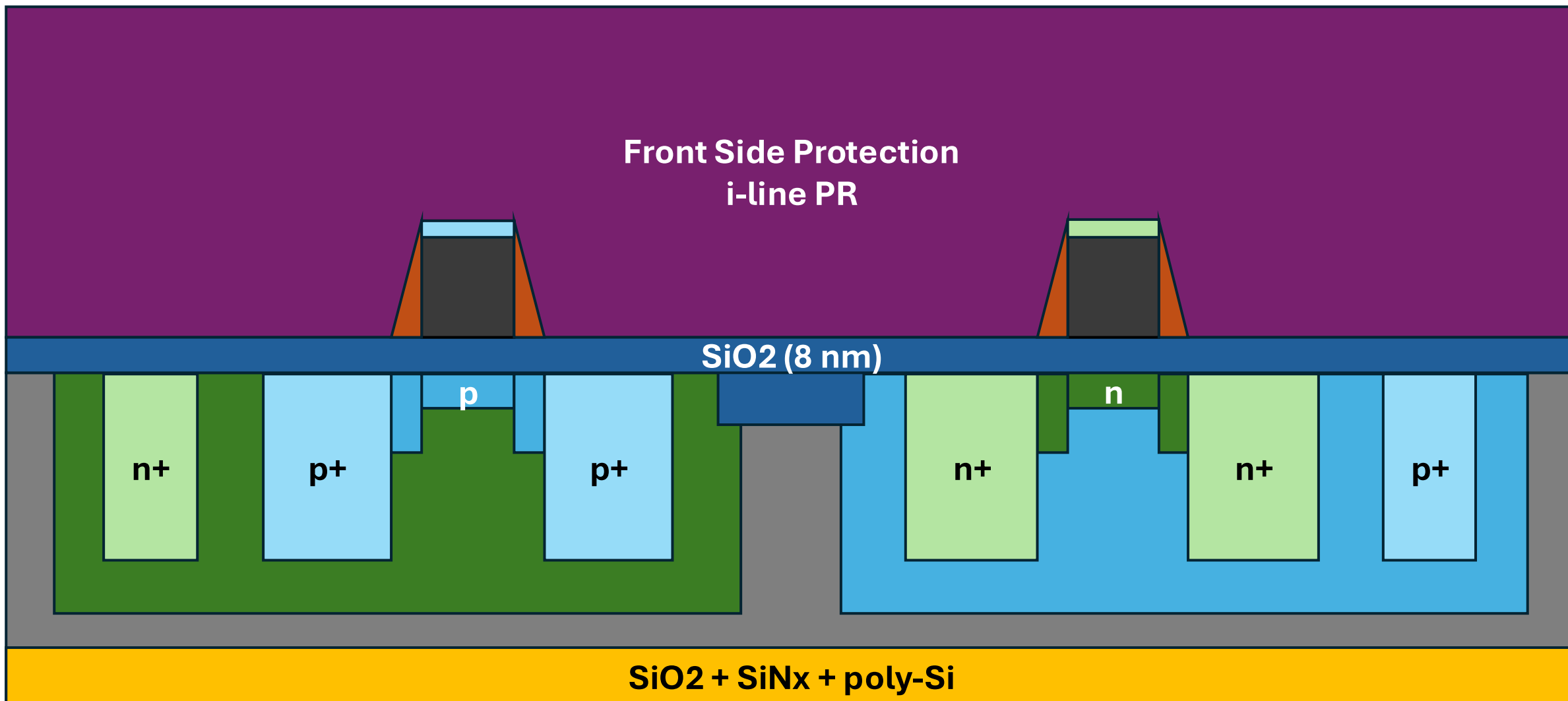
55. PR Coating for Front Side Protection
