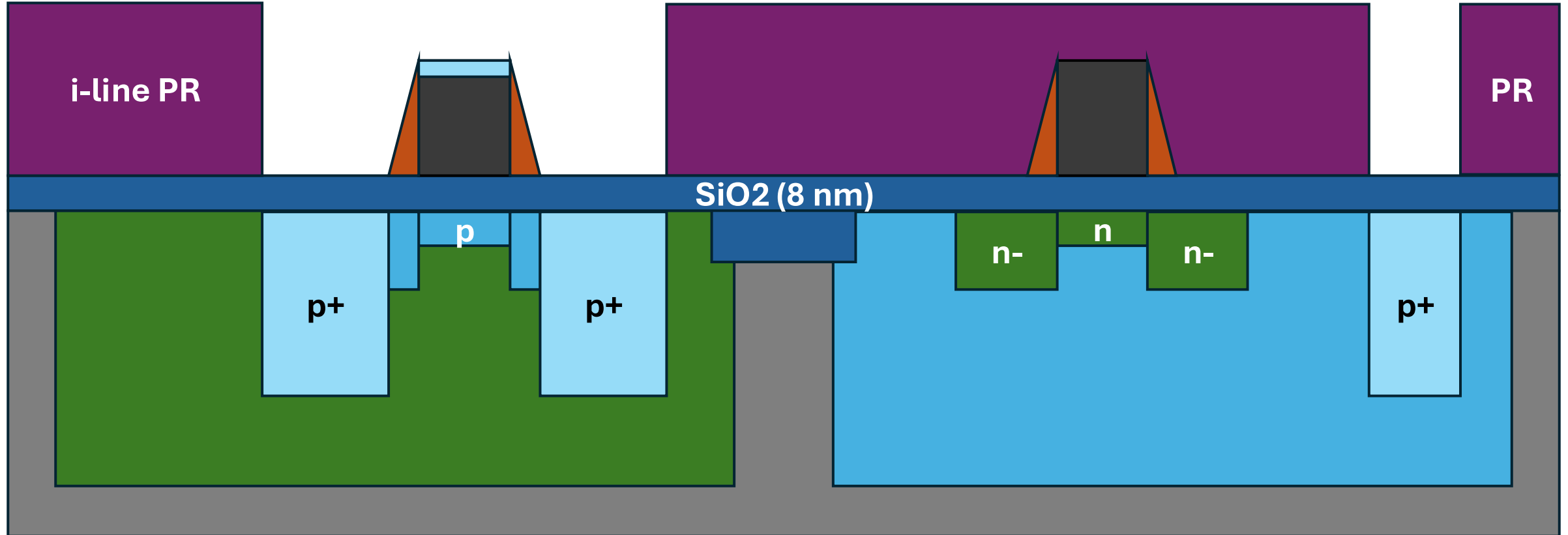
51. p+ Gate & S/D + GND Implant
