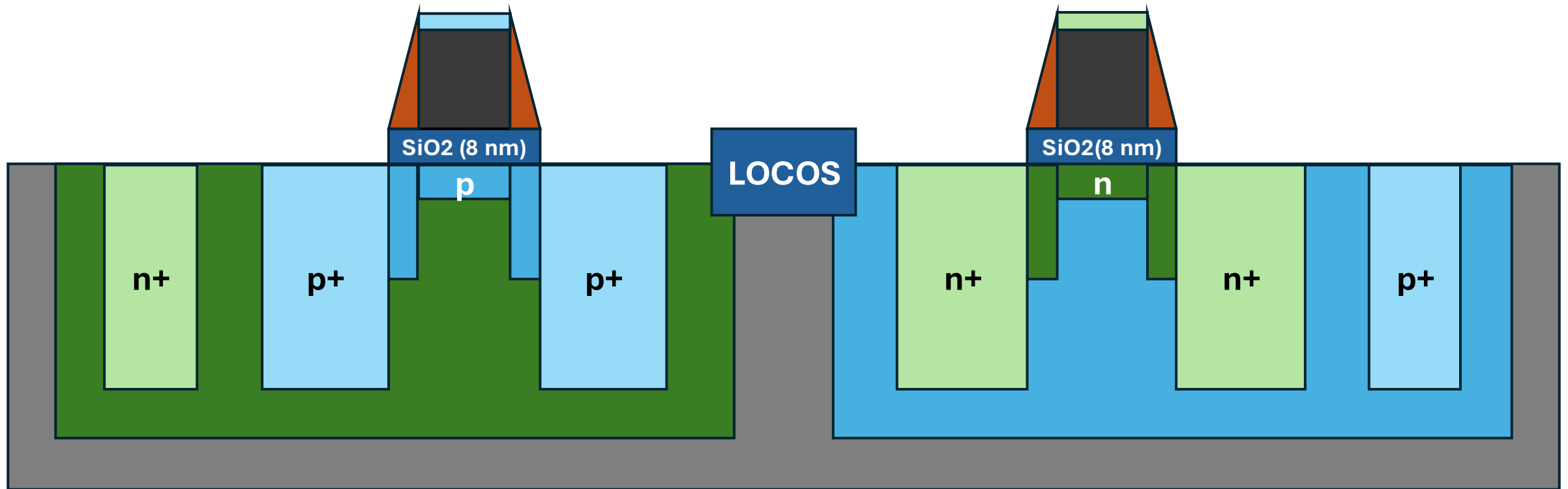
58. Sputter Etch
