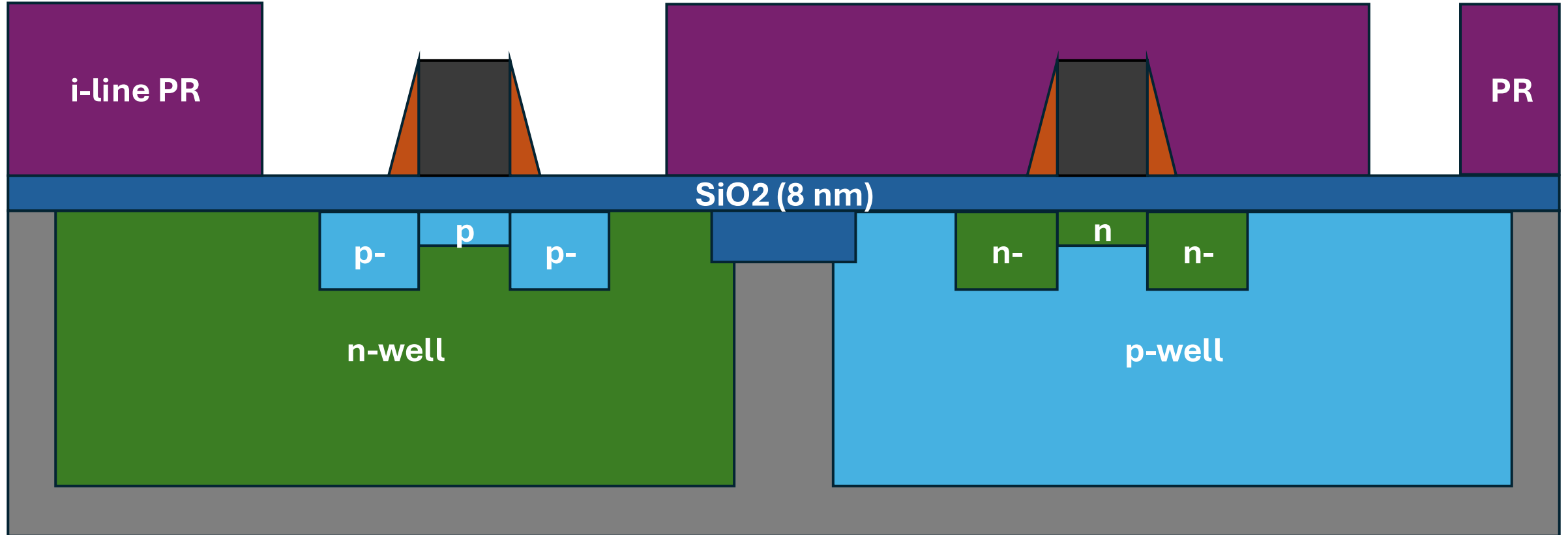
50. p+ Gate & S/D + GND Implant Litho
