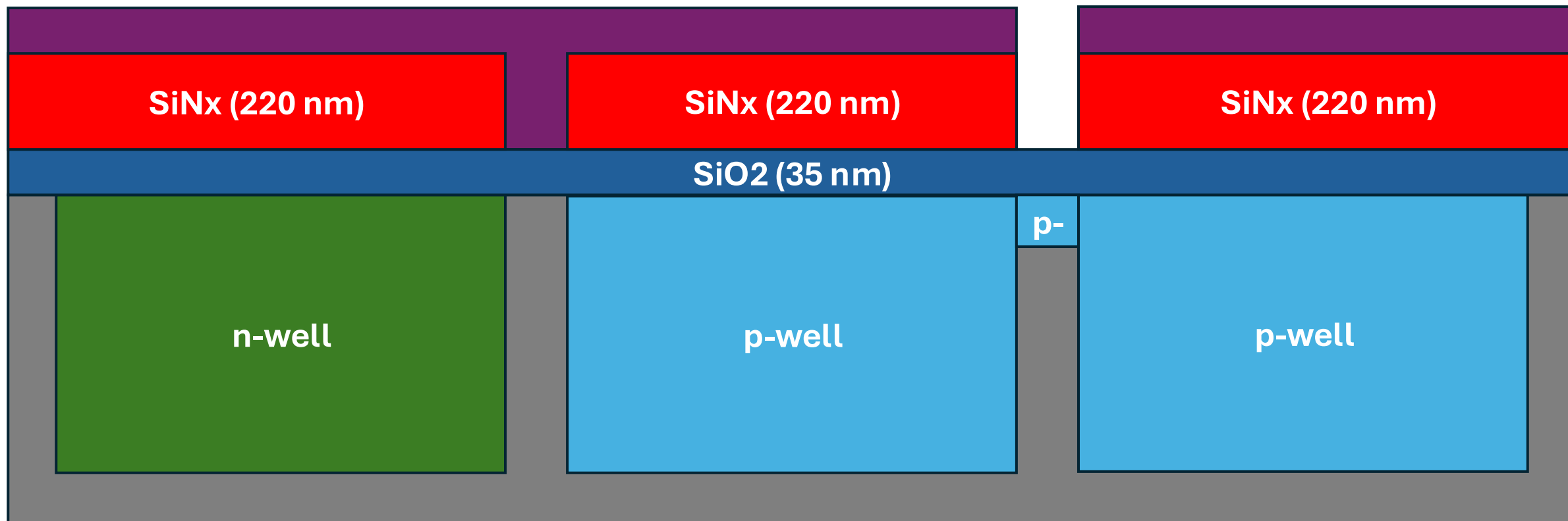
25. p-well Field Implant
