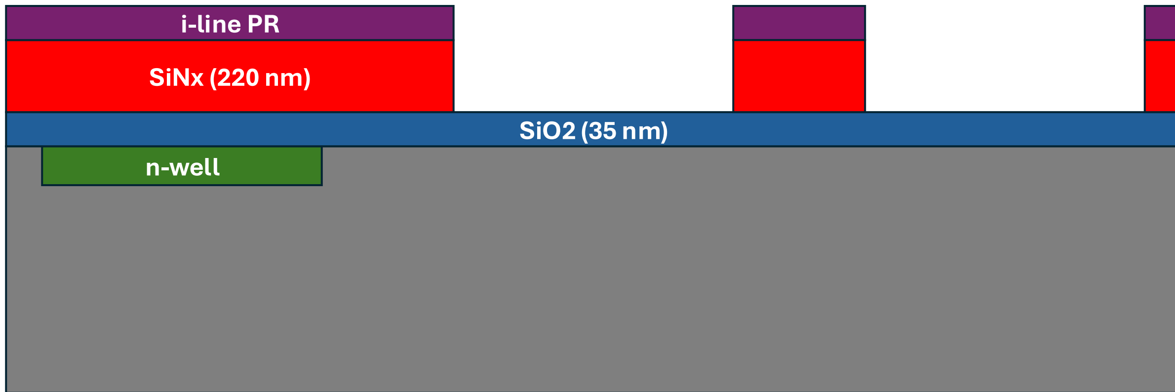
15. Nitride Dry Etch
