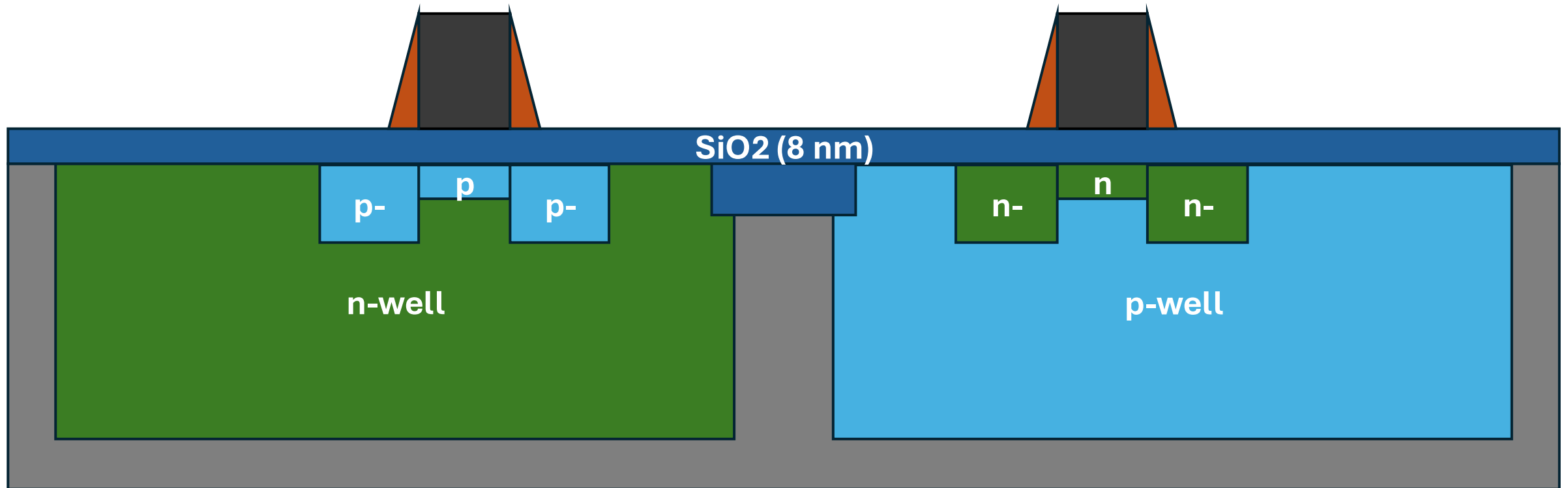
49. Spacer Formation (Blanket Etch)
