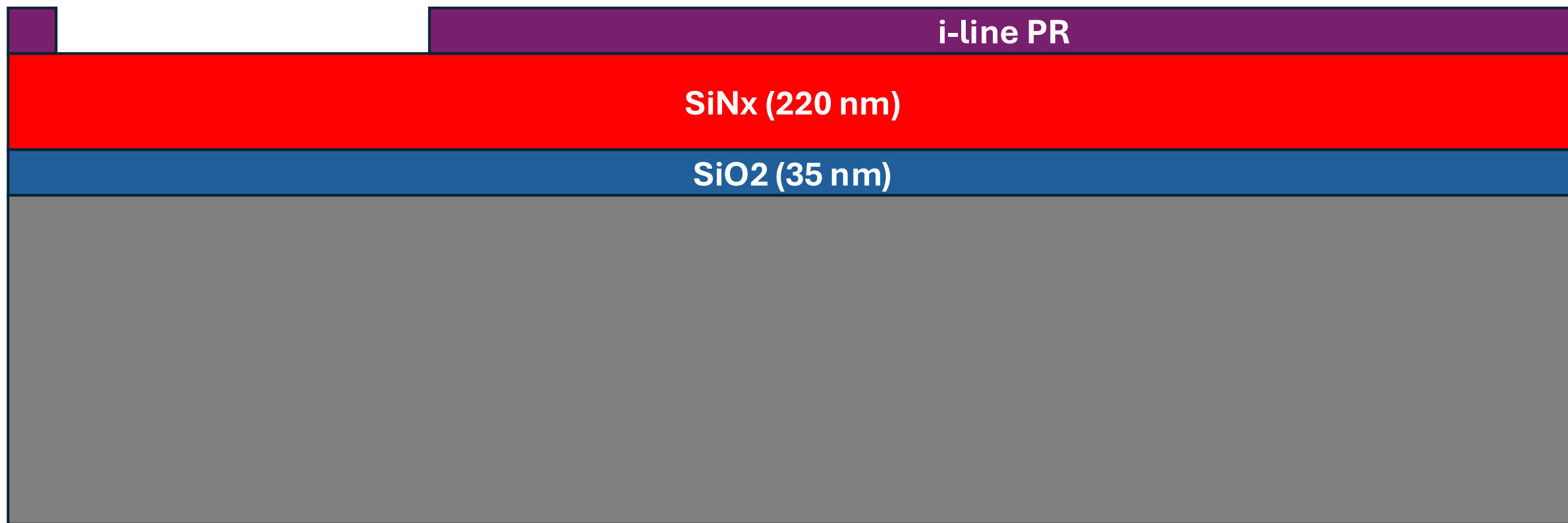
9. n-well Litho
