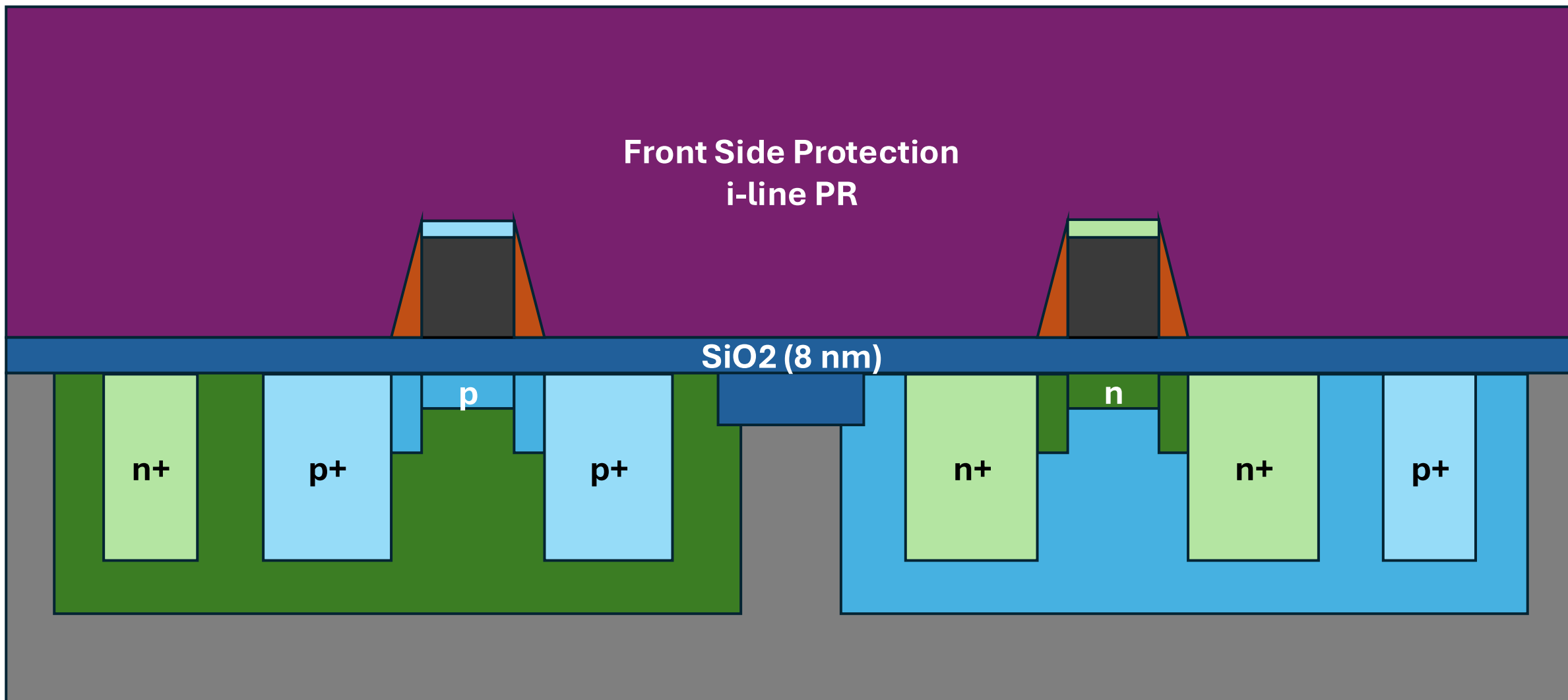
56. Oxide + Nitride + poly-Si Etch
