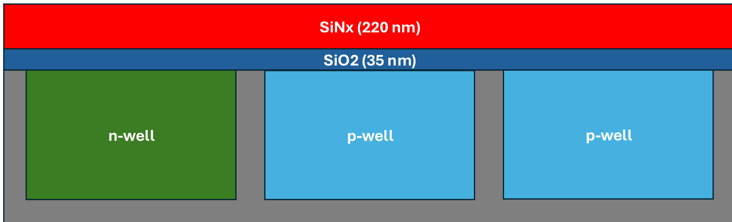
20. Oxide + Nitride Deposition
