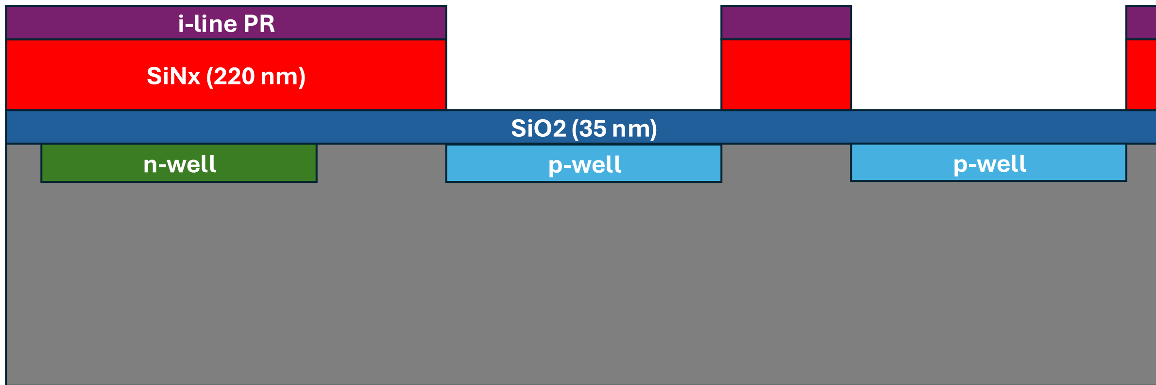
16. p-well Implantation
