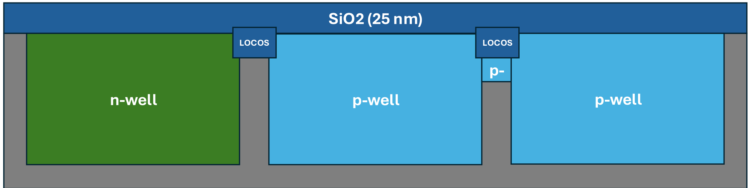
29. Sacrificial Oxidation
