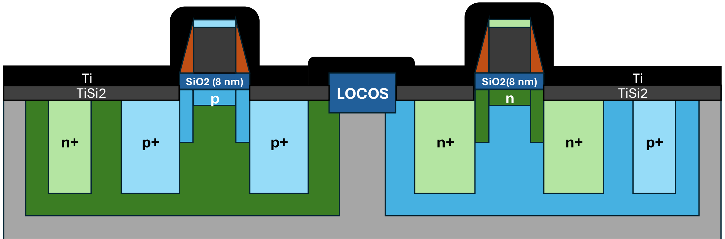
60. RTA – Silicidation (TiSi2) [N2 Chamber]
