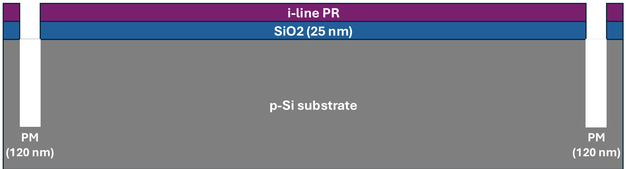
5. PM Marks Dry Etch
