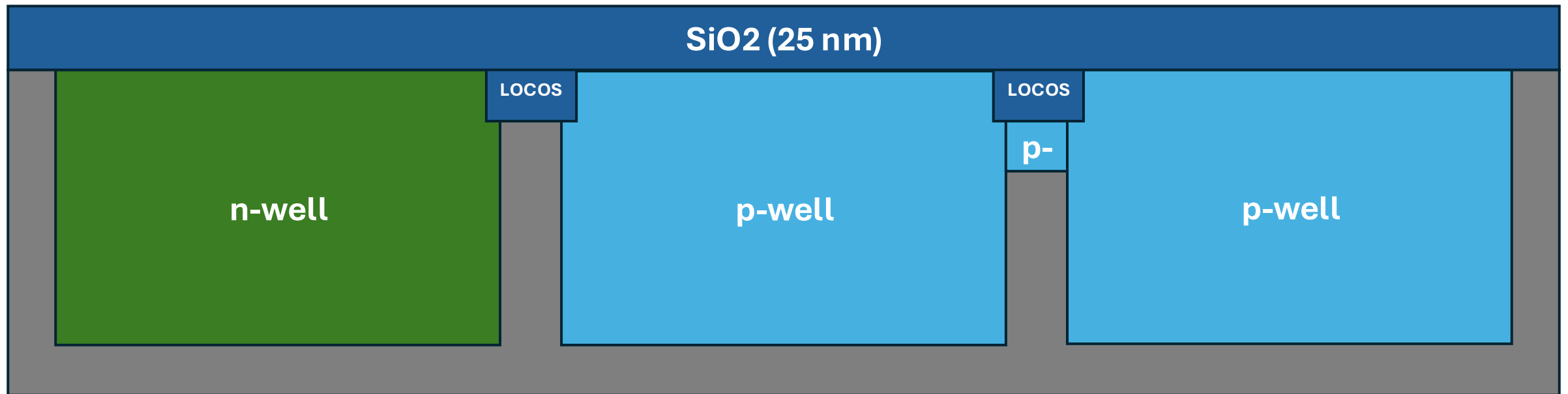
31. Screen Oxidation
