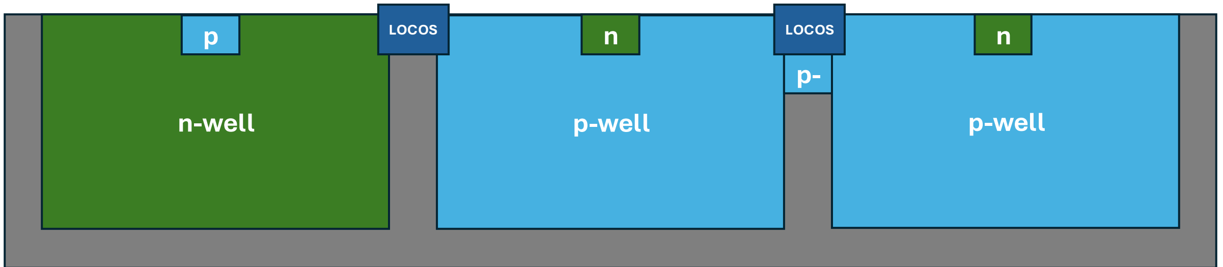
37. PR Strip + Oxide Removal
