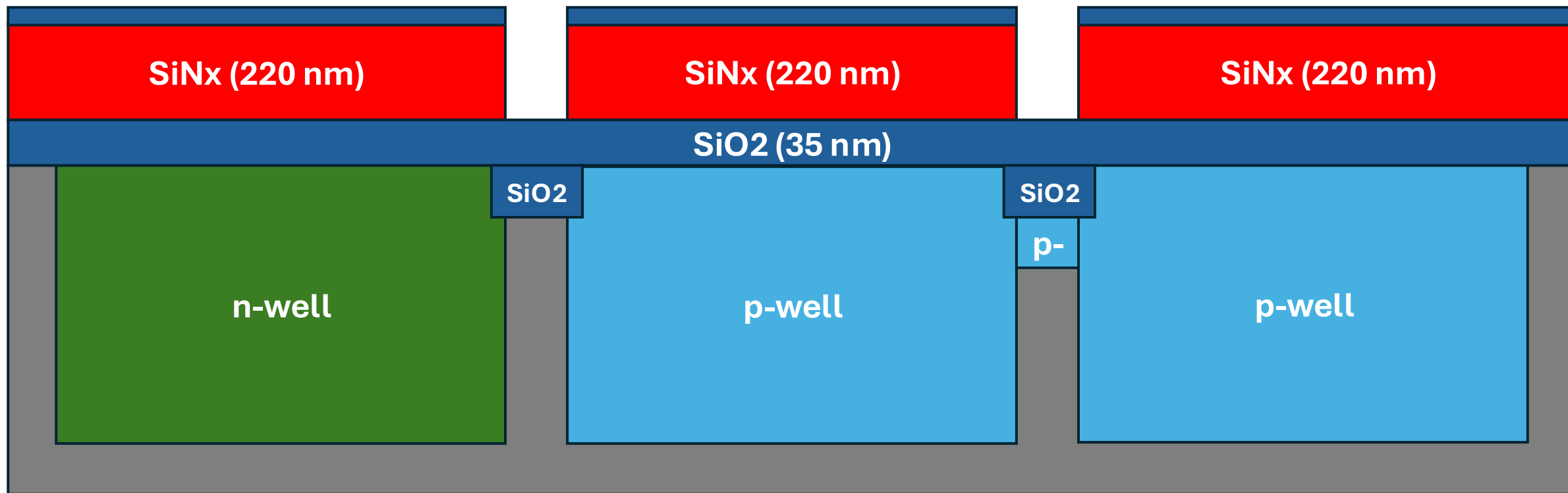
27. LOCOS (550 nm)
