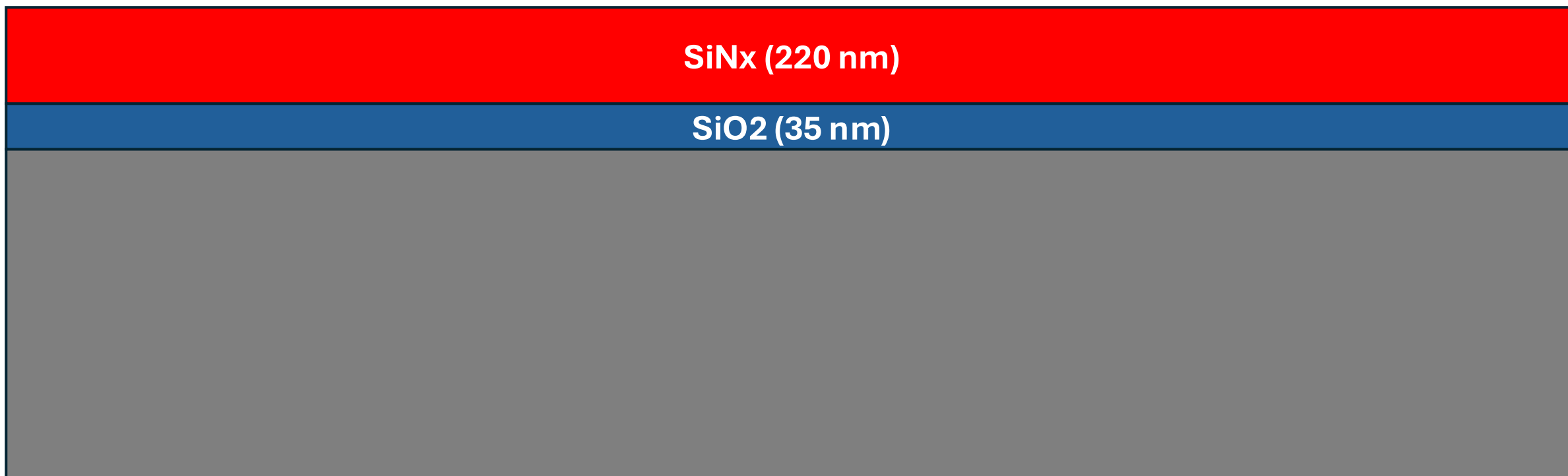
8. Pad Oxide + Nitride Deposition
