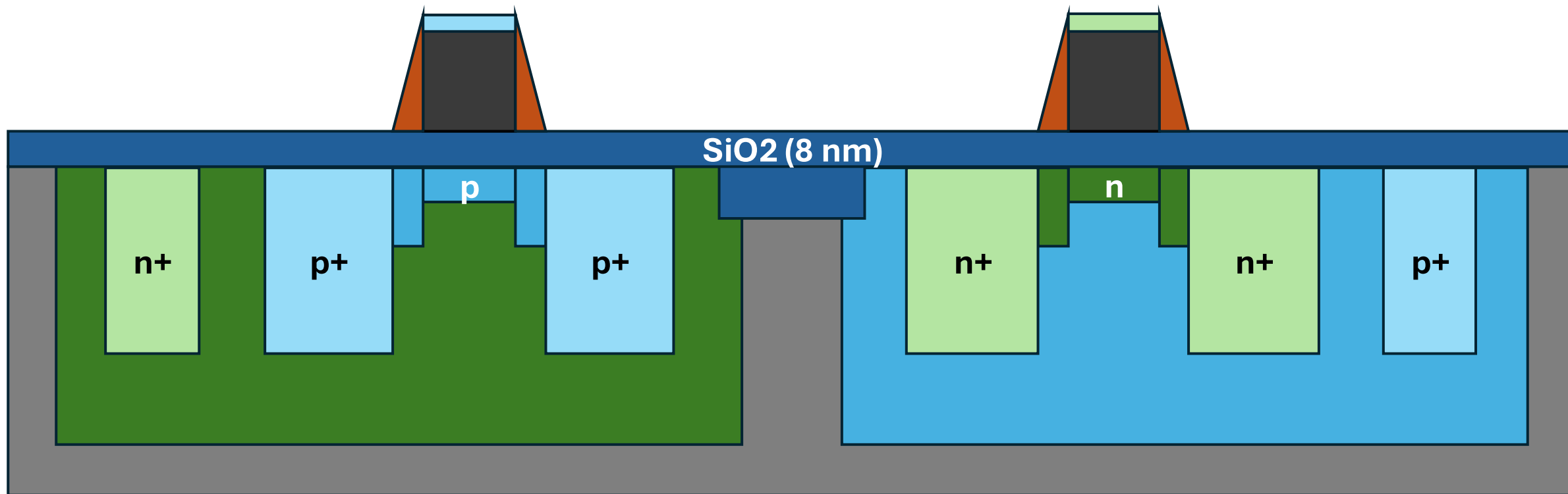
54. PR Strip
