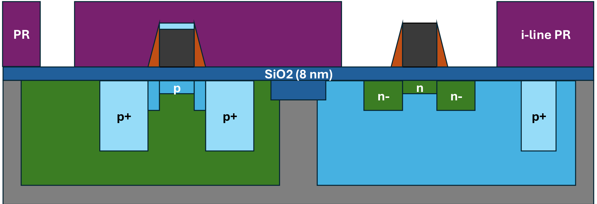
52. n+ Gate & S/D + GND Implant Litho
