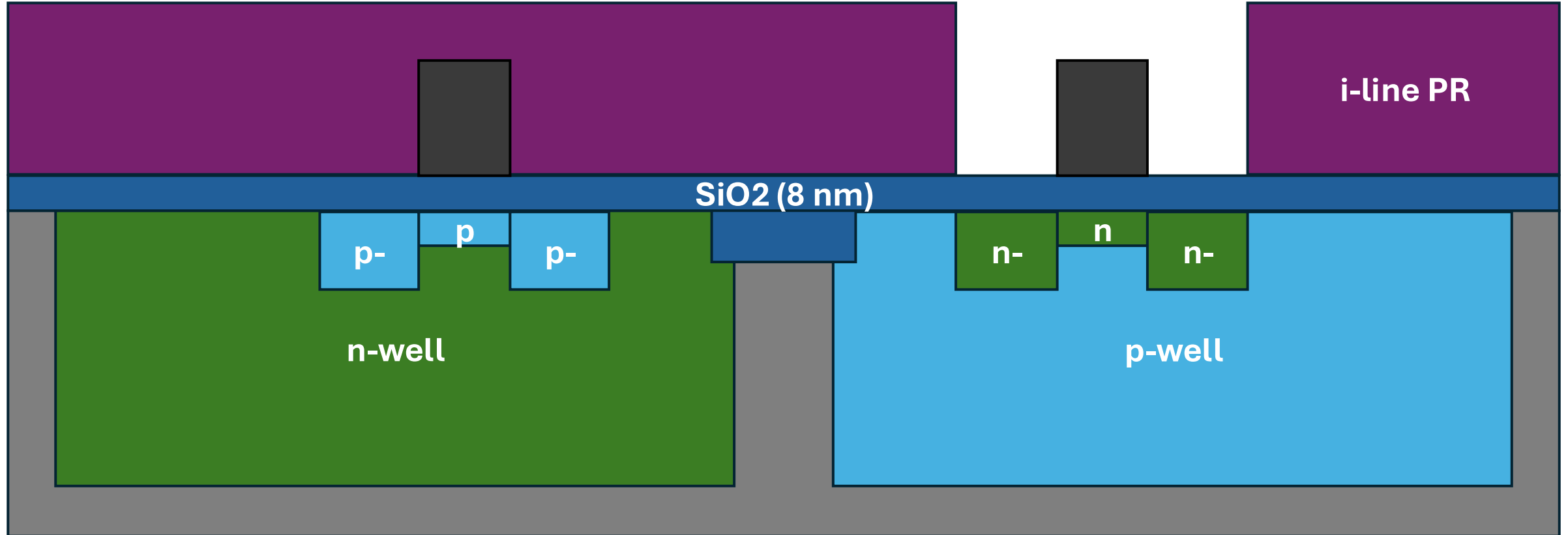
46. NMOS LDD Implant
