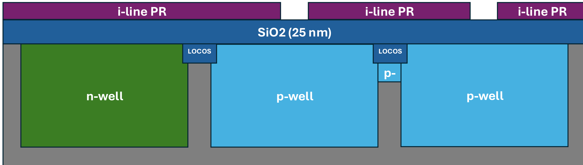
32. NMOS Vt Implant Litho
