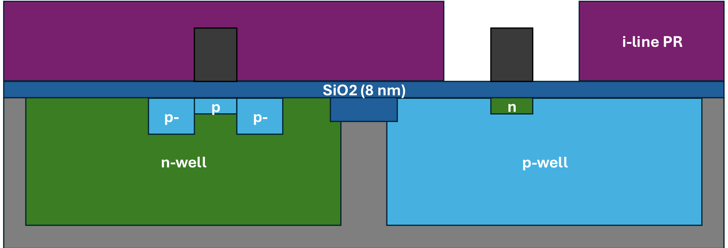
45. NMOS LDD Implant Litho
