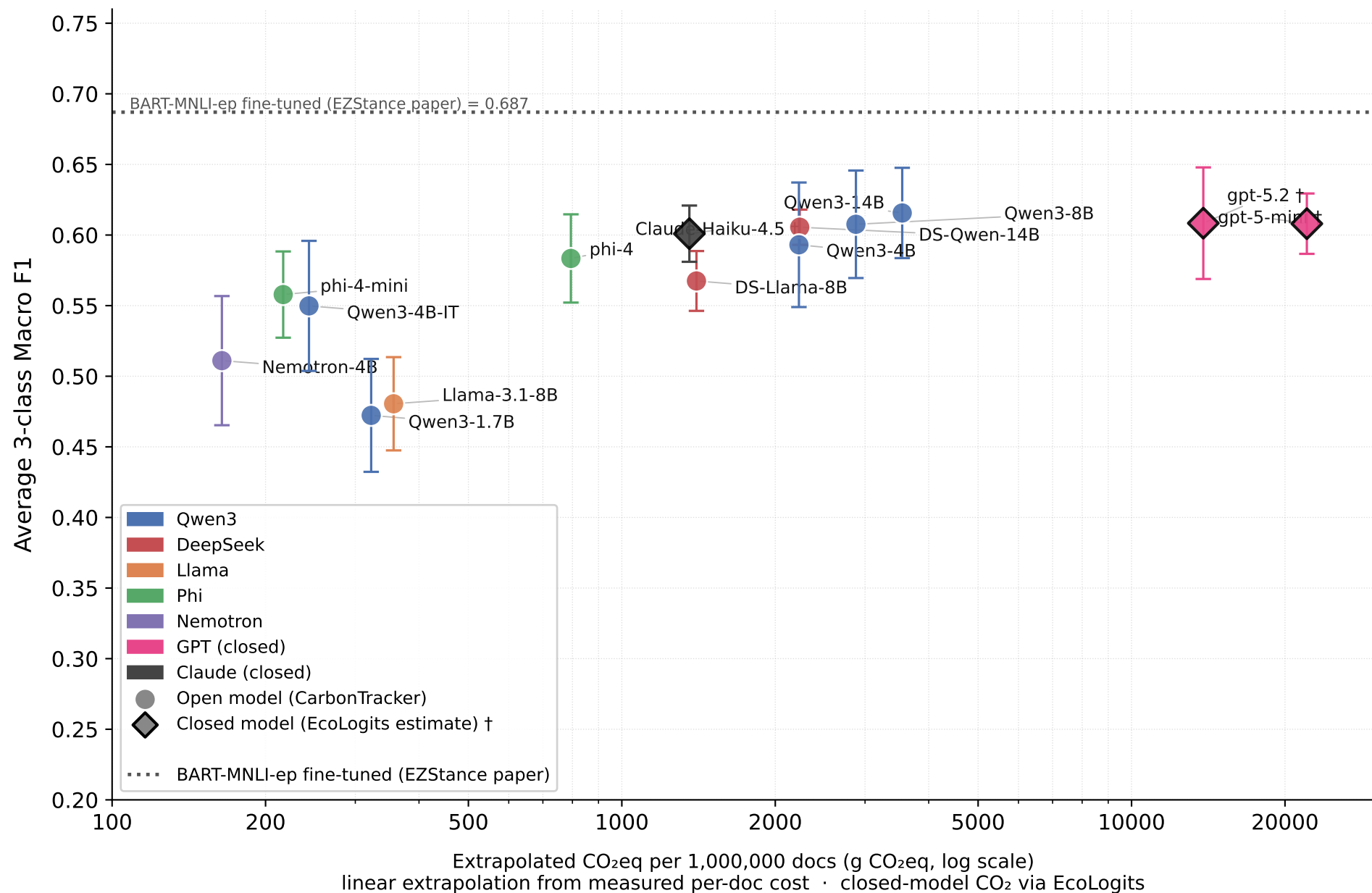
EZStance — Performance vs Carbon Cost at 1M-doc Scale
