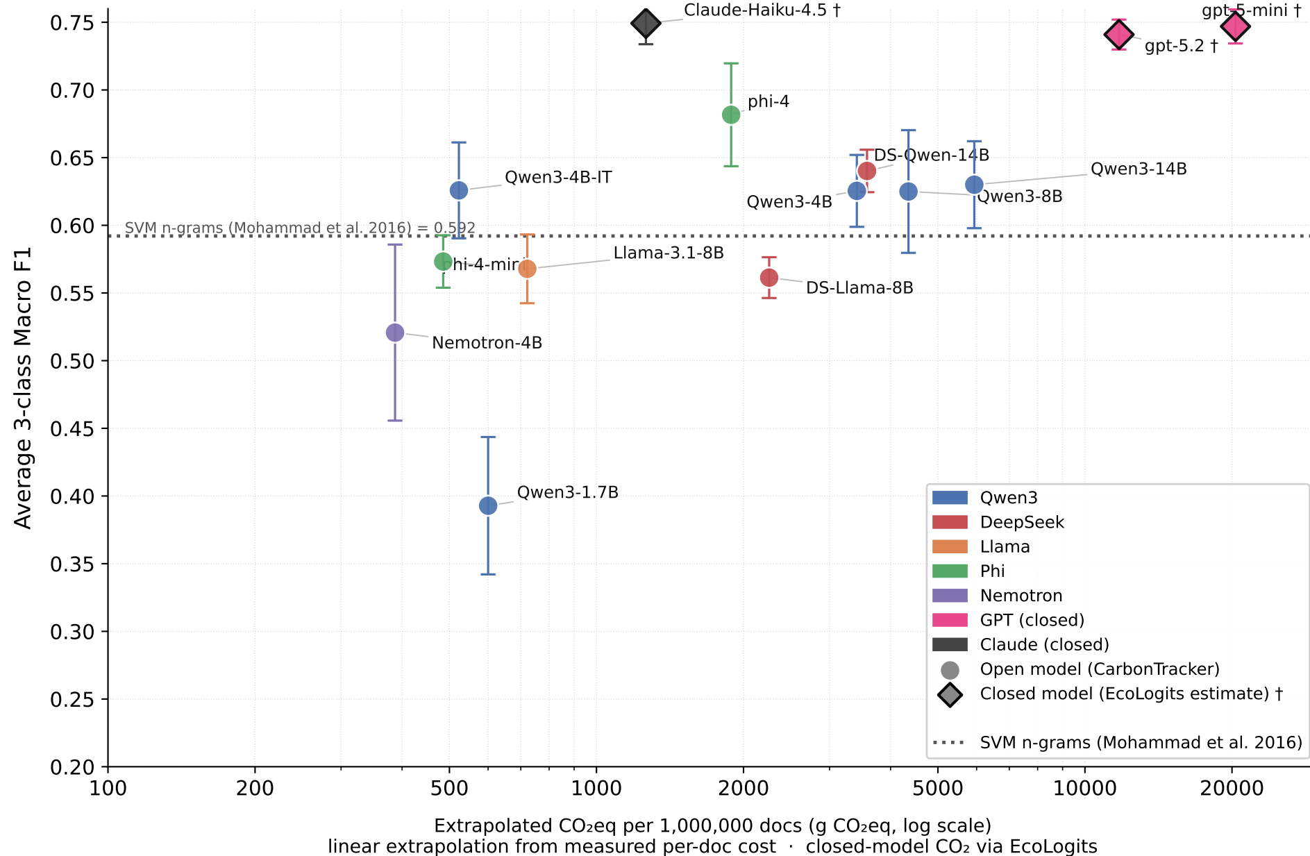
SemEval 2016 — Performance vs Carbon Cost at 1M-doc Scale
