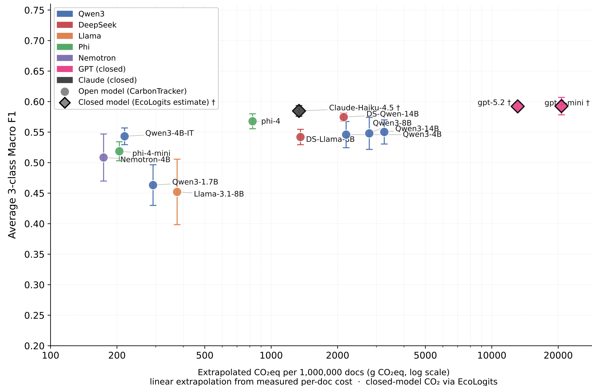
MTCSD — Performance vs Carbon Cost at 1M-doc Scale
