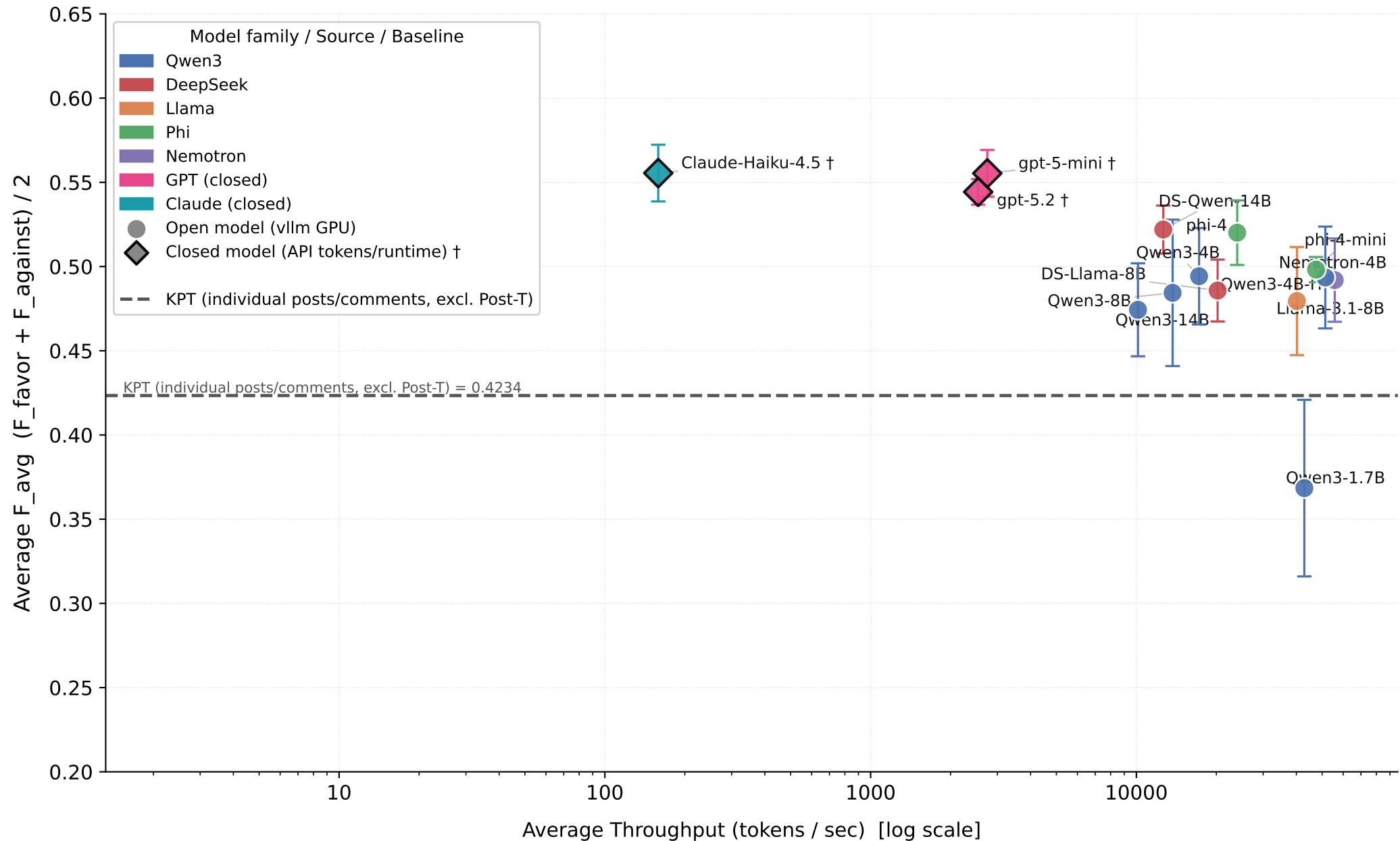
MTCSD — Throughput vs Performance [2-class F_avg, excl. Post-T, with error bars]
