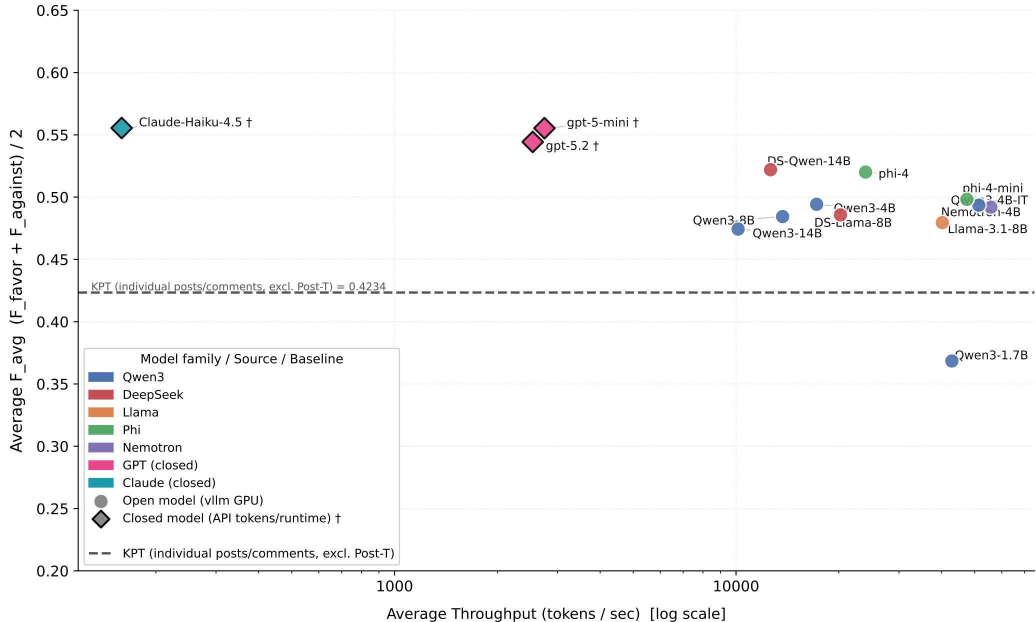
MTCSD — Throughput vs Performance [2-class F_avg, excl. Post-T, average only]
