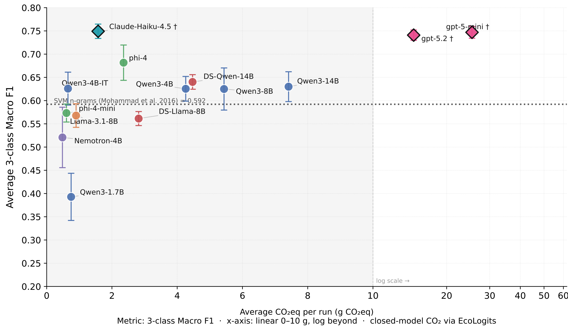
SemEval 2016 — Performance vs Carbon Cost
