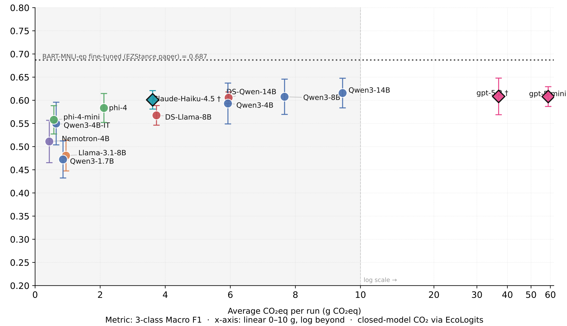
EZStance — Performance vs Carbon Cost
