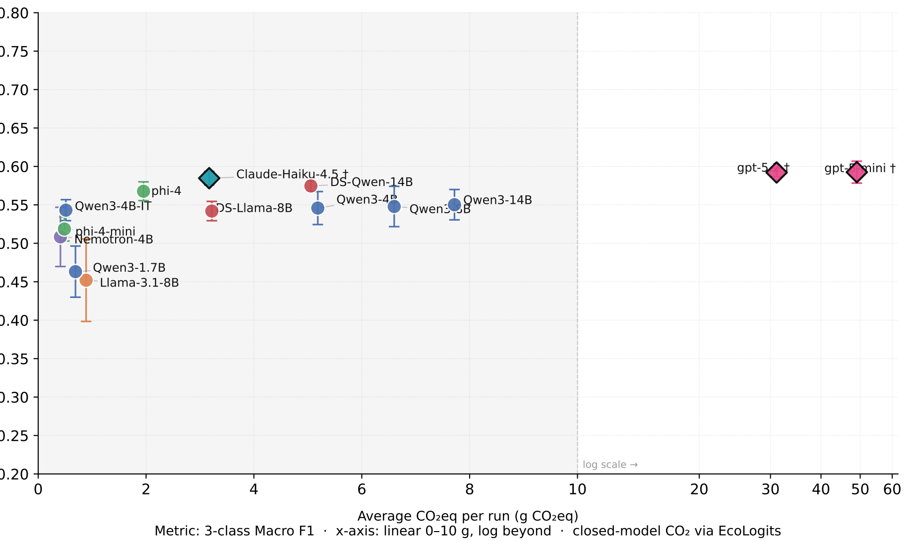
MTCSD — Performance vs Carbon Cost
