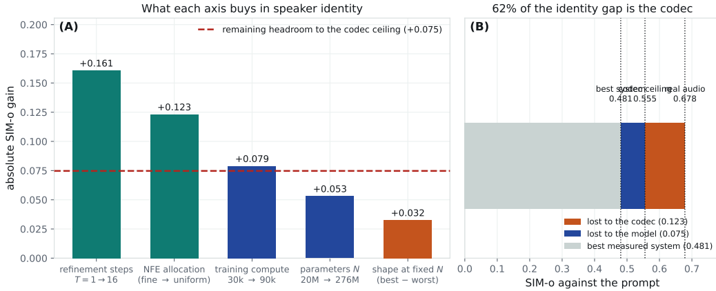
Figure 4: Identity is mostly not the model's to win. (A) what each axis buys in speaker similarity, against the headroom that remains to the codec ceiling. (B) of the distance between real audio and our best system, 62% is lost in the codec itself.
