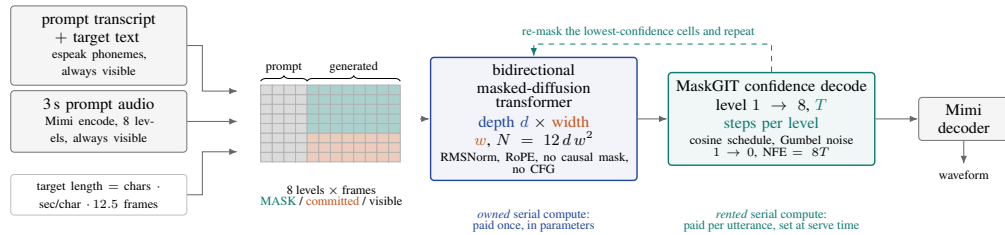
Figure 1: The two ways a masked-diffusion TTS model buys sequential computation. Phonemes and a 3-second prompt are always visible; the generated region of the 8 \times frames token grid starts fully masked. The backbone spends depth — owned serial compute, fixed at training time — and the sampler spends T refinement steps per codebook level — rented serial compute, chosen at serve time. One training grid over (w, d) therefore yields a whole (w, d, T) surface at inference. This paper asks whether the rented kind helps every capability equally.
