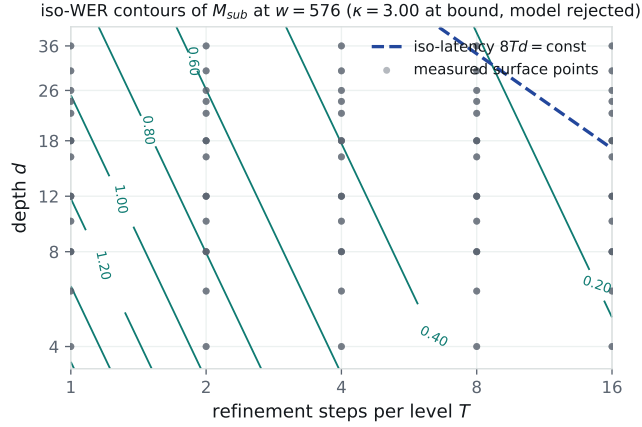
Figure 5: Why the substitution form is rejected. Iso-WER contours of M_{\text{sub}} in (\log T, \log d) at the median width, with the iso-latency line 8Td = \text{const} . The fitted \kappa sits on its bound and \Delta\text{AICc}(M_{\text{sub}} - M_{\text{sep}}) = +69.3 , so these contours are shown as a rejected model, not as a design rule.
