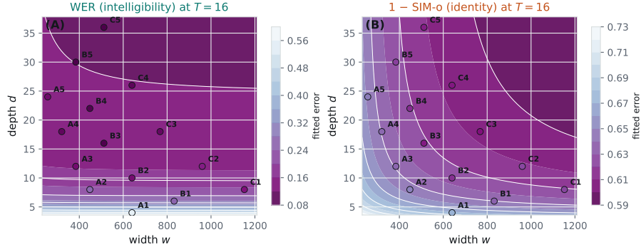
Figure 6: Fitted anisotropy surface at T=16 for both metrics, with the measured config means overlaid. The width amplitude A saturates its pre-registered upper bound for both metrics, which is why \rho = \alpha/\beta is reported as unidentified in §4 even though the two-axis model beats the N -only model ( \Delta\text{AICc} = -15.5 and -5.5 ).
