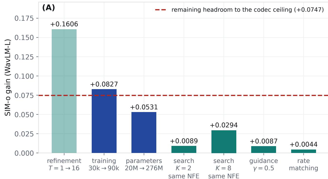
SIM-o gain of each change
