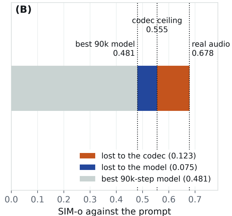
62% of the gap to real audio is the codec
