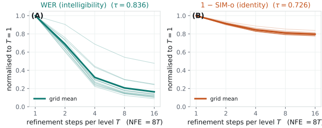
Figure 3: Test-time scaling is metric-selective. Error versus refinement steps for all 15 configs, each normalised to its own T=1 value; thick lines are grid means. (A) WER error falls 0.952 in absolute terms over T=1 \rightarrow 16 and is still falling at T=16 . (B) SIM-o error falls 0.161 over the same range, 5.9\times less. Same models, same frozen sampler, same items — only T differs.
