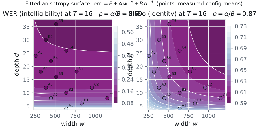
Figure 4: Fitted anisotropy surface at T=16 for both metrics, with the measured config means overlaid. The width amplitude A saturates its pre-registered upper bound for both metrics, which is why \rho = \alpha/\beta is reported as unidentified in §4 even though the two-axis model beats the N -only model ( \Delta\text{AICc} = -15.5 and -5.5 ).
