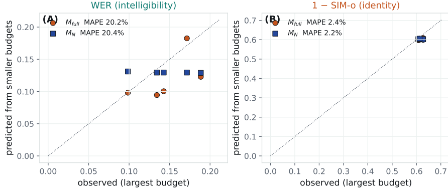
Figure 6: H-D4 extrapolation . The two smaller budgets are fitted and the largest budget predicted, under M_{\text{full}} and the N -only model. SIM-o extrapolates (MAPE 2.4 % vs 2.2 %); WER does not (20.2 % vs 20.4 %).
