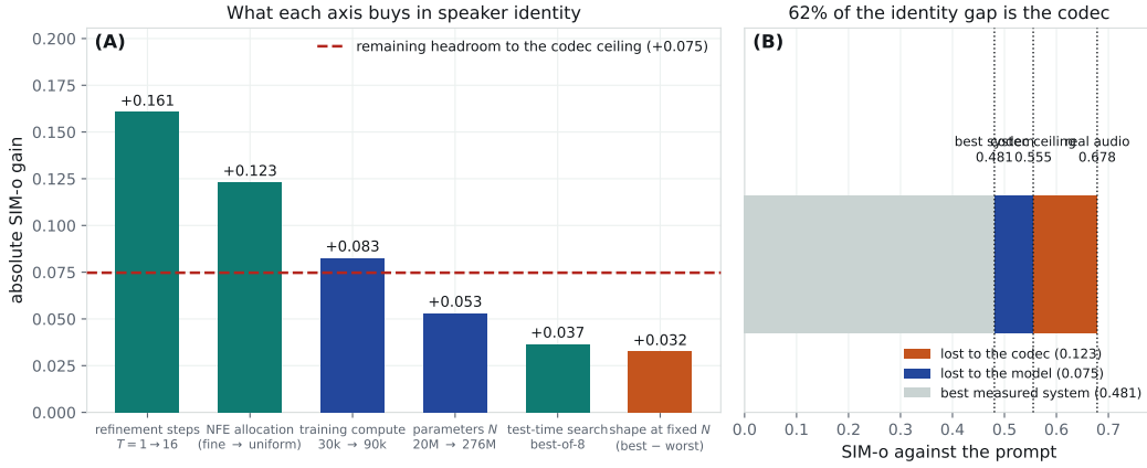
Figure 3: Identity is mostly not the model's to win. (A) what each axis buys in speaker similarity, against the headroom that remains to the codec ceiling; bars are coloured by which lever they are (rented at serve time, owned in training, shape). Refinement's bar is the largest only because it is measured from one-step decoding, which is not an operating point anyone ships; from the deployable T=16 default it buys nothing further, and test-time search is what moves identity from there. (B) of the distance between real audio and our best system, 62% is lost in the codec itself.
