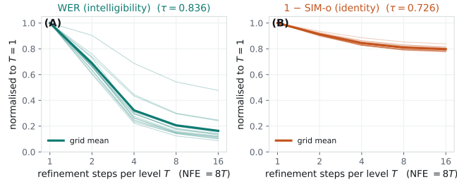
Figure 4: Test-time scaling is metric-selective . Error versus refinement steps for all 15 configs, each normalised to its own T=1 value; thick lines are grid means. (A) WER error falls 0.952 in absolute terms over T=1 \rightarrow 16 and is still falling at T=16 . (B) SIM-o error falls 0.161 over the same range, 5.9\times less. Same models, same frozen sampler, same items — only T differs.
