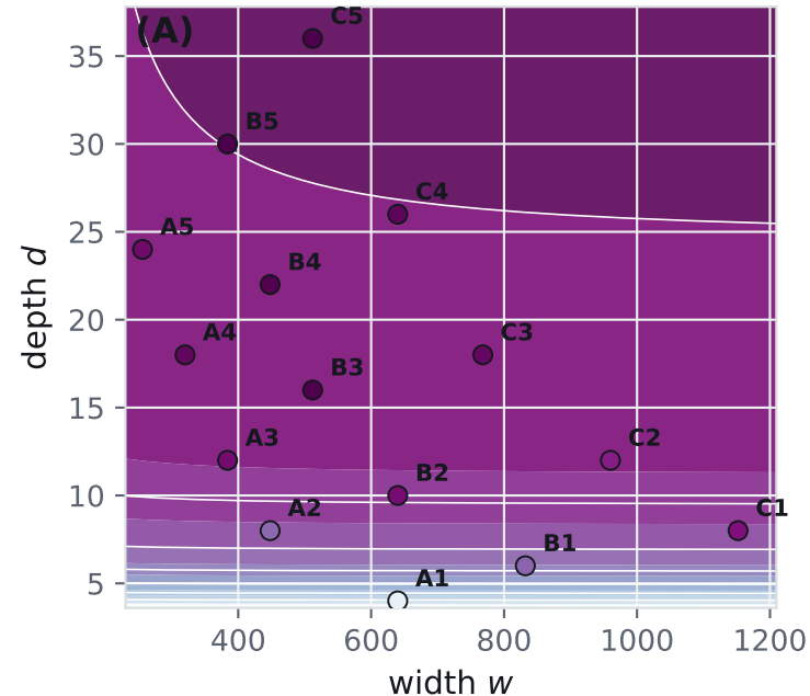
WER (intelligibility) at T = 16
