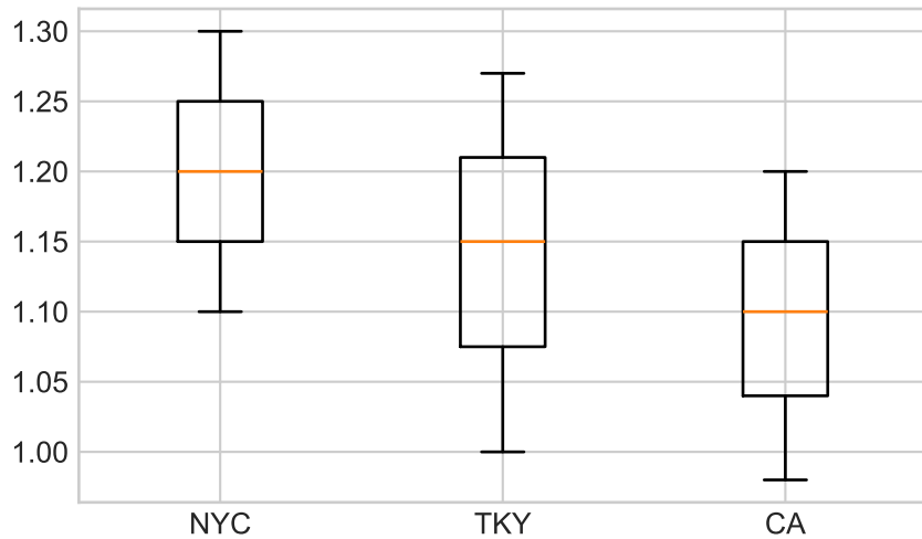
Entropy (Mock)
