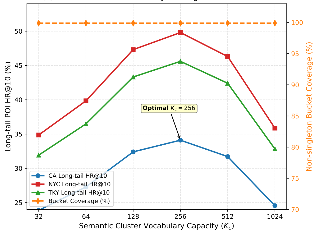
(c) Semantic Cluster Number K_c vs. Long-tail Generalization
