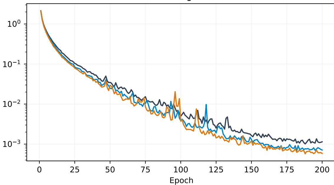
Training CE
