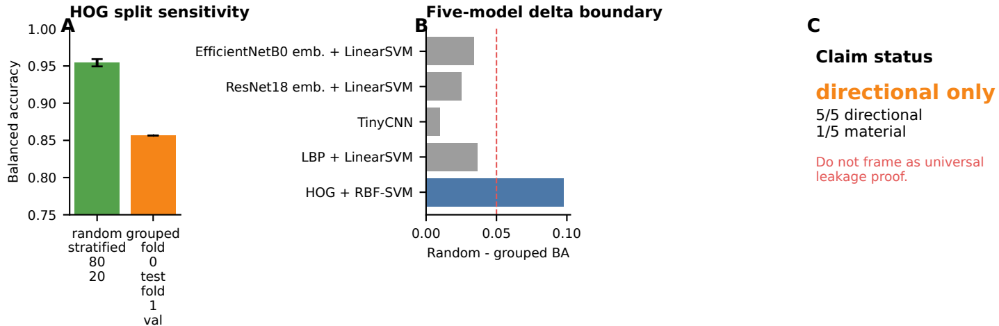
Figure 3 preview | Mojahid split effect is modest and model-dependent
