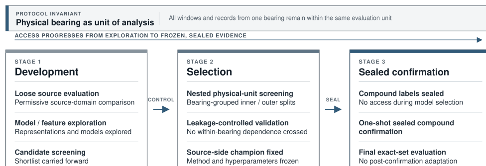
Figure 1. The SCGP access ladder. Evaluation progresses from exploratory source-domain development, through leakage-controlled physical-unit selection, to one-shot sealed compound confirmation. P0 and P1 are deliberately loose diagnostic states. From P2 onward, the physical bearing is the invariant unit: all windows and records derived from one bearing remain within the same evaluation partition.
