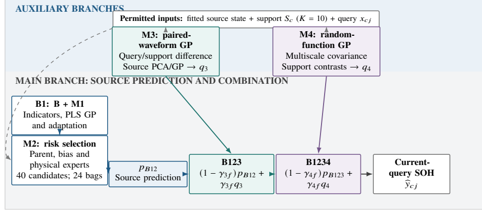
Figure 2: Support-conditioned prediction combination. M1 and M2 form the source-prediction path. M3 and M4 each produce an SOH estimate from source-fitted state, early target support and the current query; these estimates are successively blended with the parent prediction. Solid arrows carry predictions and dashed arrows indicate input information. The branch estimates are not fitted to parent-model residuals.
