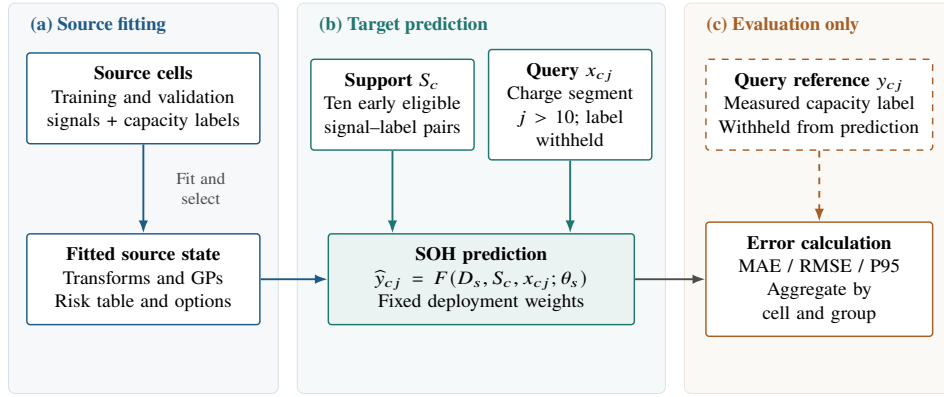
Figure 1: Task and information boundary. Source fitting, target prediction and evaluation are separated. The first ten eligible target measurements and the current query signal enter prediction; the query capacity label enters error calculation only. Development scores informed architecture and global-strength selection, whereas the subsequent UL-PUR and MICH evaluations used frozen XJTU models and weights.
