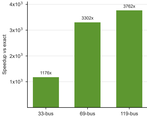
Amortized online inference
