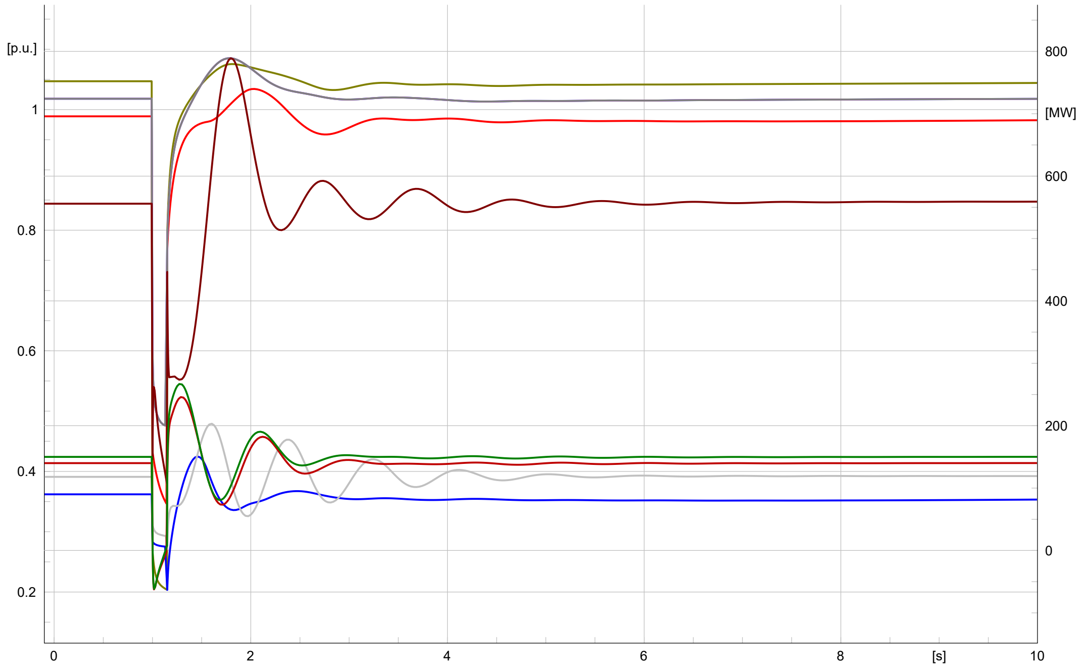
Three phase short circuit at 1s at bus 380 kV BE-Busbar_1. Short Curcuit is cleared at 1.15 s, no elements are tripped.
