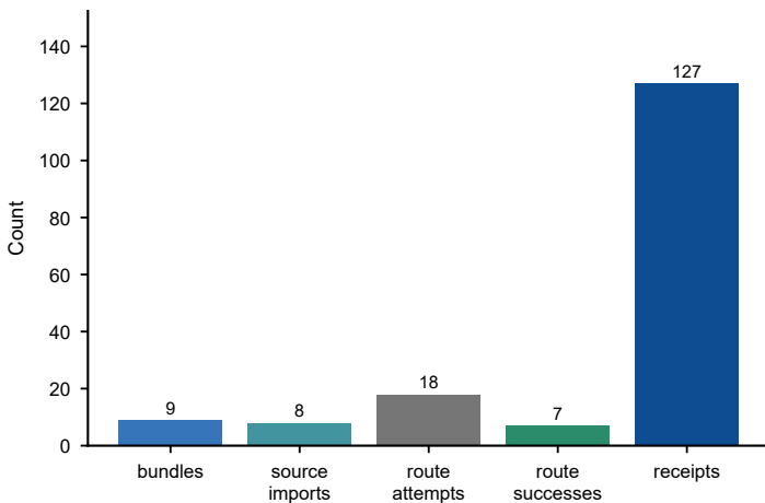
c PCC endpoint and success-criterion boundary
