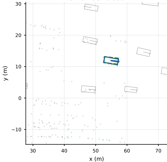
truckscenes frame 000267 target 11 (IoU gain +0.166)
