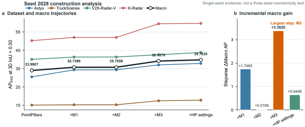
Figure 4: Progressive seed-2028 construction analysis across the four radar datasets and their macro average. Panel (a) traces AP through the PointPillars screen, M1–M3, and the final high-performance settings; bold labels mark the macro trajectory. Panel (b) reports stepwise macro changes relative to the immediately preceding configuration. This single-seed analysis explains module behavior but does not establish three-seed monotonicity.
