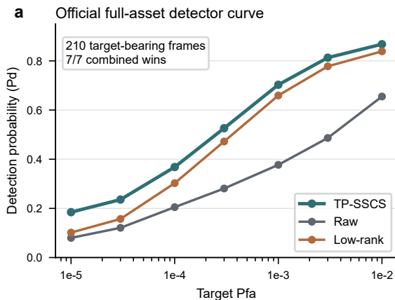
Figure 4 | Official AISTAP-SIM full-asset detector validation
