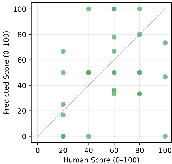
Method 2b Structured Extraction \rho = 0.177
