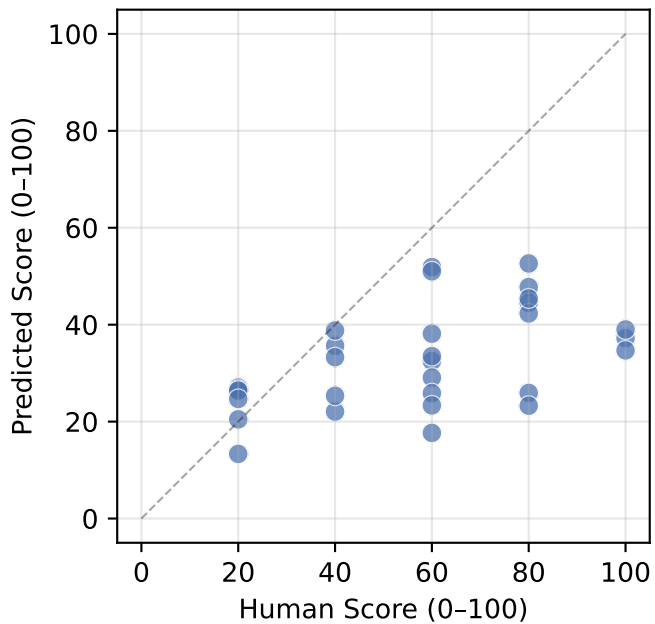
Method 2a Dense Embedding \rho = 0.517
