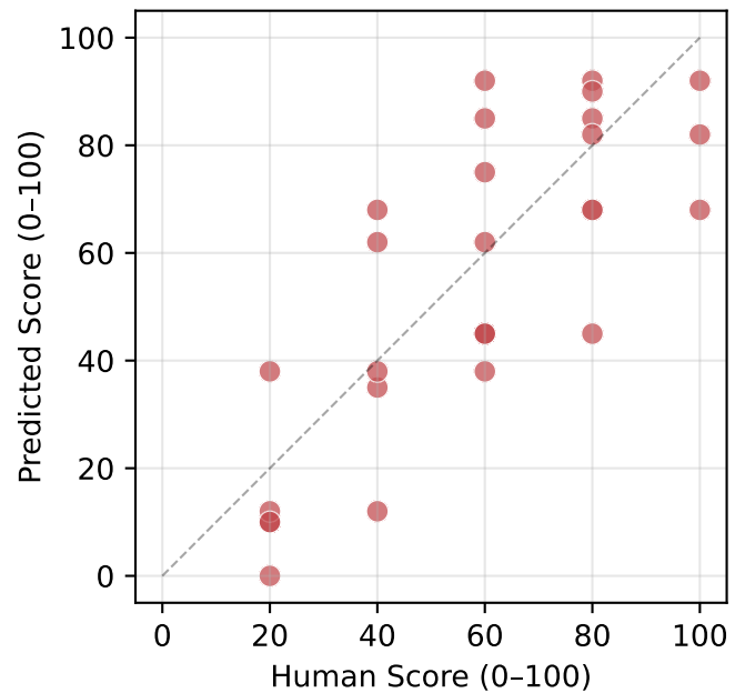
Method 2c LLM-as-Judge \rho = 0.788
