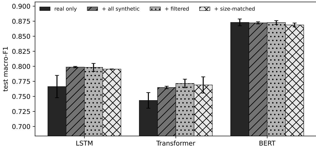
Effect of synthetic data (mean \pm std over seeds)
