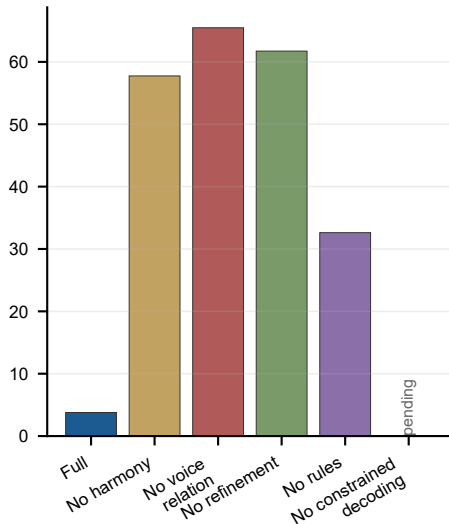
Rule flags/100
