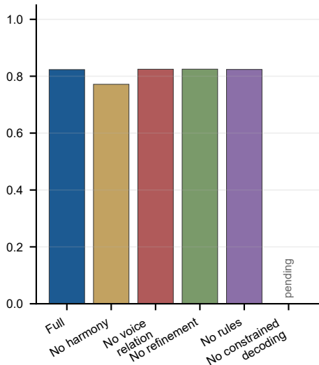
Pitch accuracy
