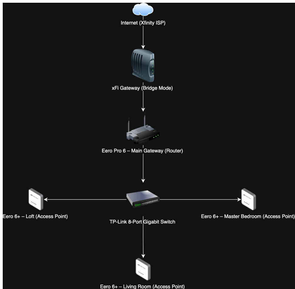
Figure 1: Home Network Topology with Wired Backhaul
