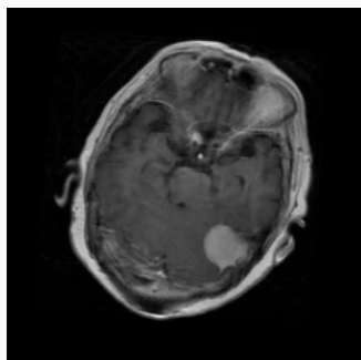
Original MRI
