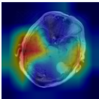
Grad-CAM
