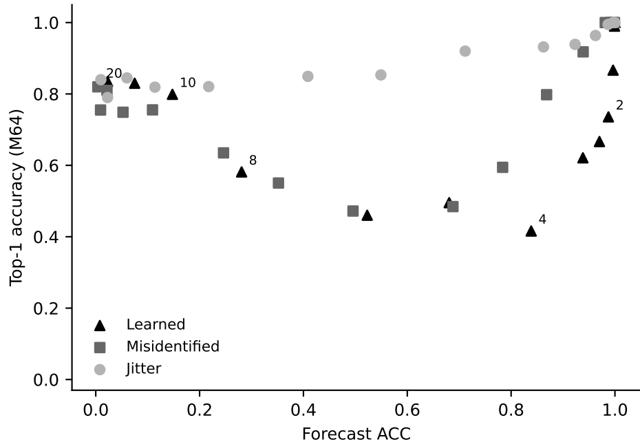
Lorenz-96
