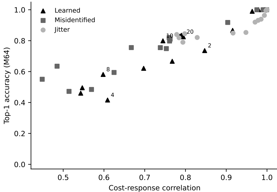
Lorenz-96
