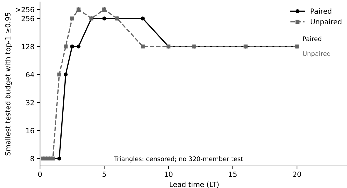
Lorenz-96
