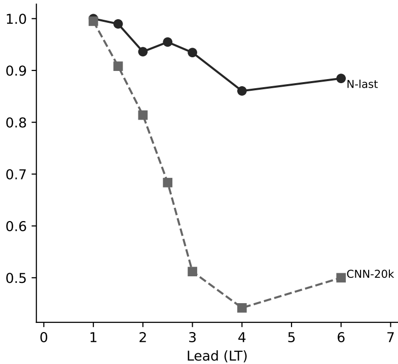
Eligible best-action accuracy
