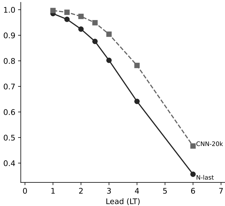
Decision-window ACC
