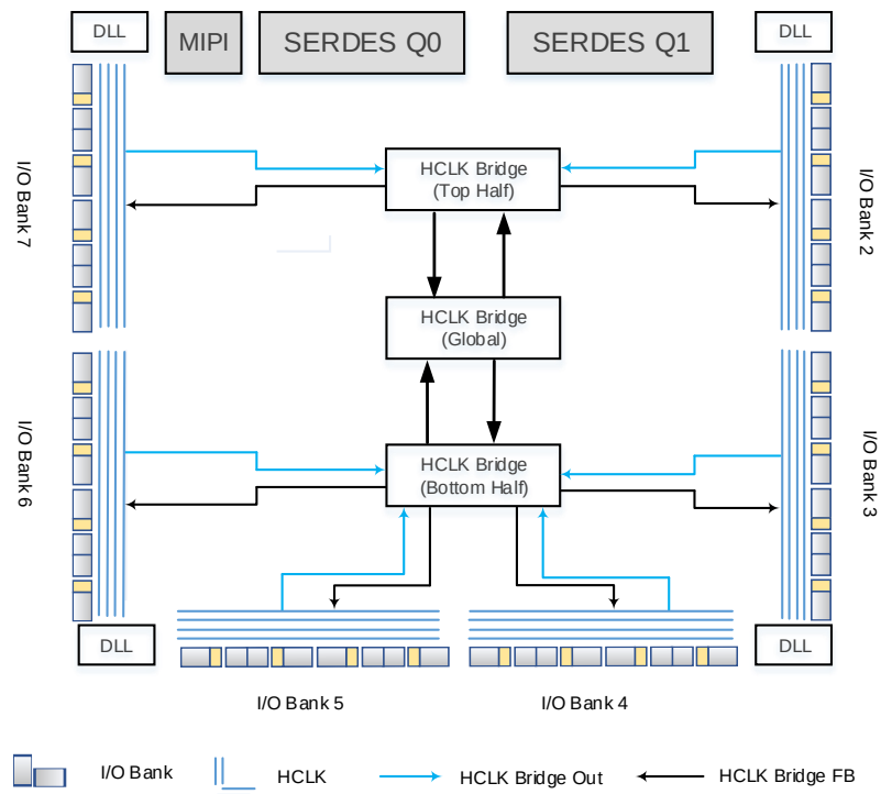
Figure 2-6 HCLK Structure View (60K)
