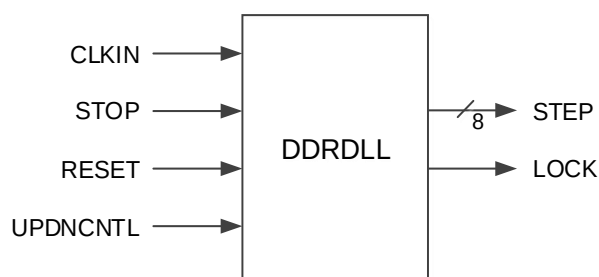
Figure 5-12 DDRDLL Port Diagram
