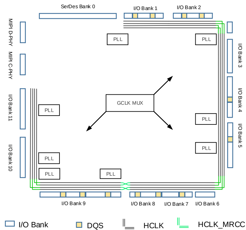
Figure 2-3 Clock Resources (25K)
