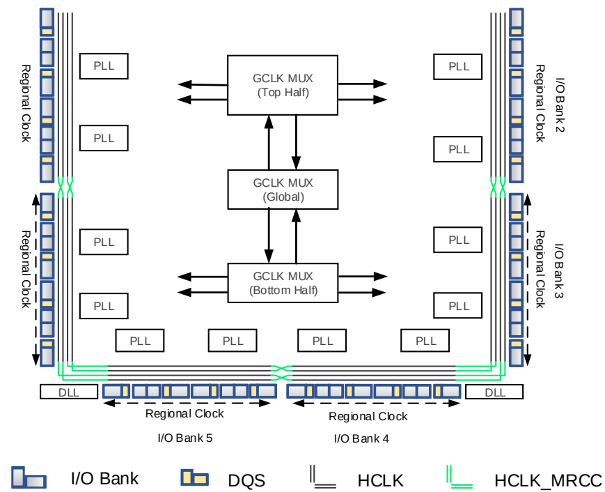
Figure 2-2 Clock Resources (60K)
