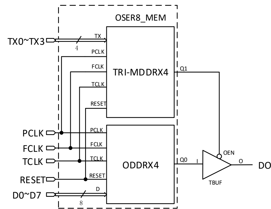
Figure 4-42 OSER8_MEM Logic Diagram
