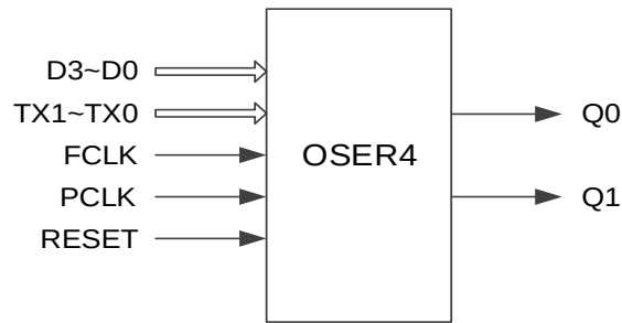
Figure 4-32 OSER4 Port Diagram
