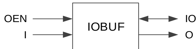
Figure 3-8 IOBUF Port Diagram
