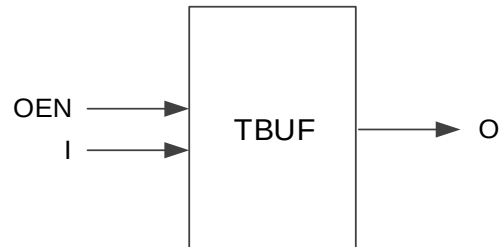
Figure 3-7 TBUF Port Diagram
