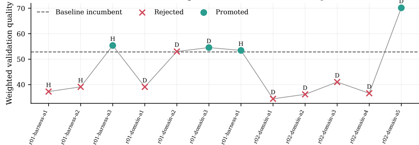
Strict co-evolution gate filters most candidate updates
