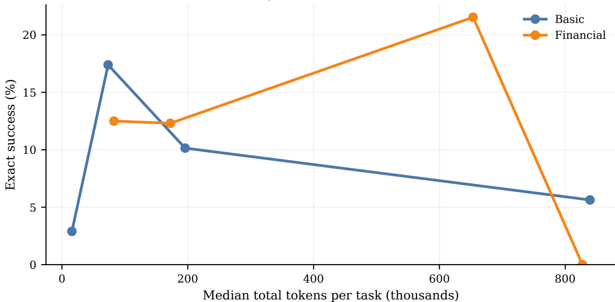
Token-accuracy relationship is non-monotonic
