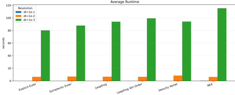
Figure 13: Average Integrator Runtime
