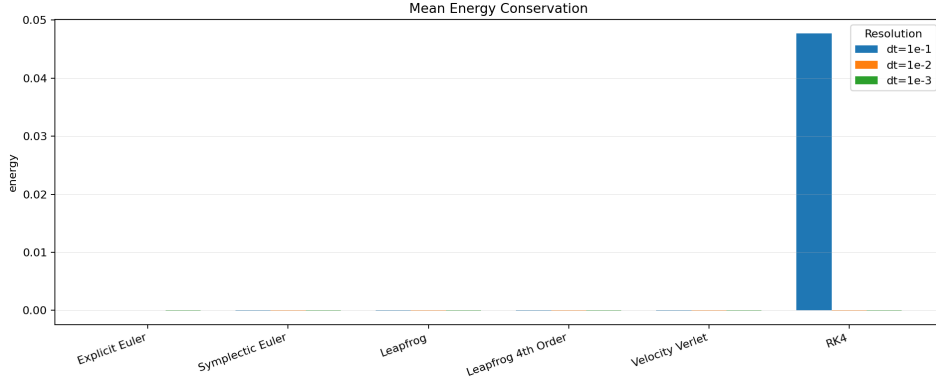
Figure 19: Mean Energy Conservation by Integrator and Resolution
