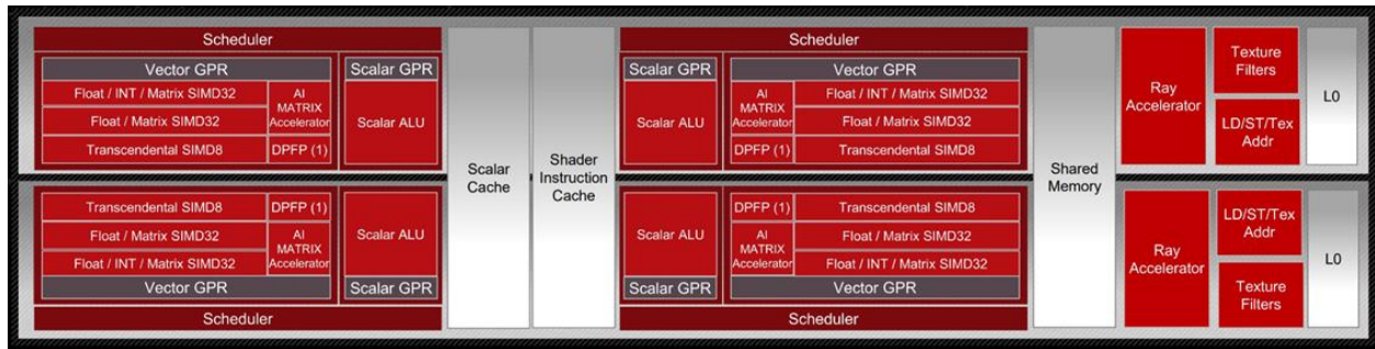
Fig. 6.3: Block Diagram of an RDNA3 work group processor.
