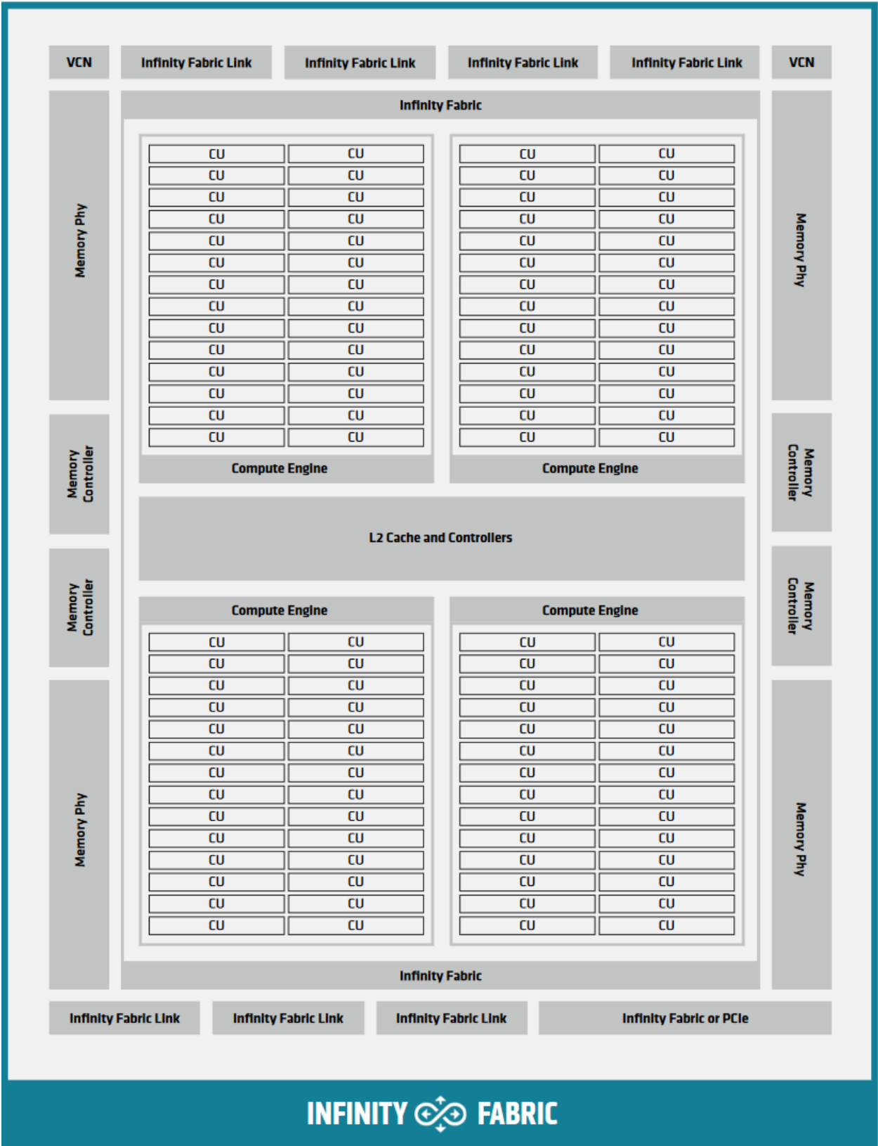
Fig. 4.3: Block Diagram of a CDNA2 Graphics Compute Die.
