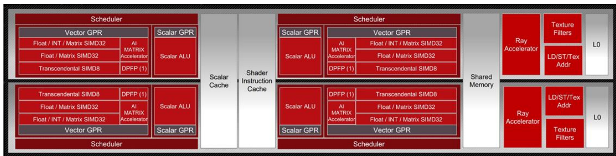
Fig. 4.1: Block Diagram of an RDNA3 Compute Unit.
