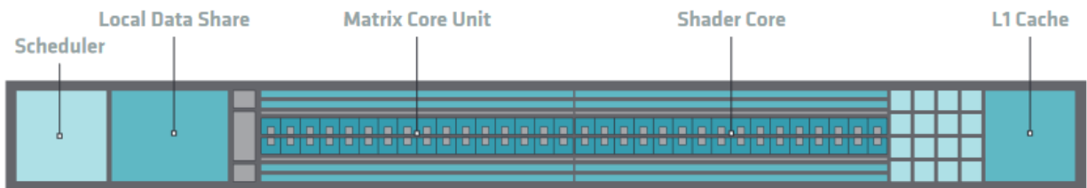
Fig. 6.2: Block Diagram of a CDNA3 Compute Unit.
