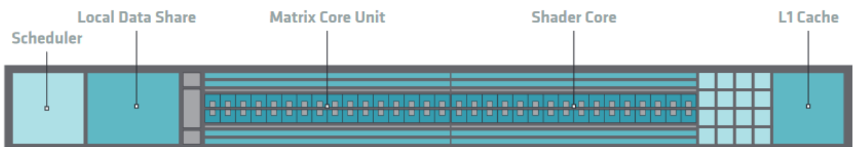
Fig. 4.2: Block Diagram of a CDNA3 Compute Unit.
