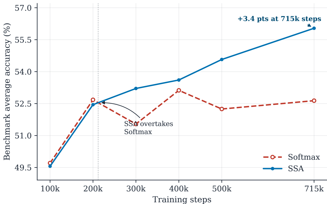
SSA vs. Softmax — aggregate benchmark accuracy across training (28-task average, English + French benchmarks)
