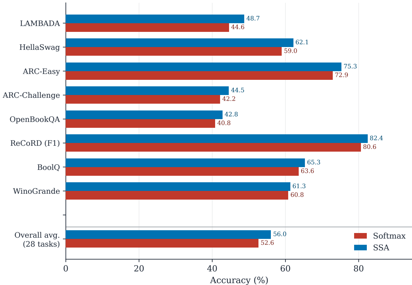
Final comparison at 715k training steps
