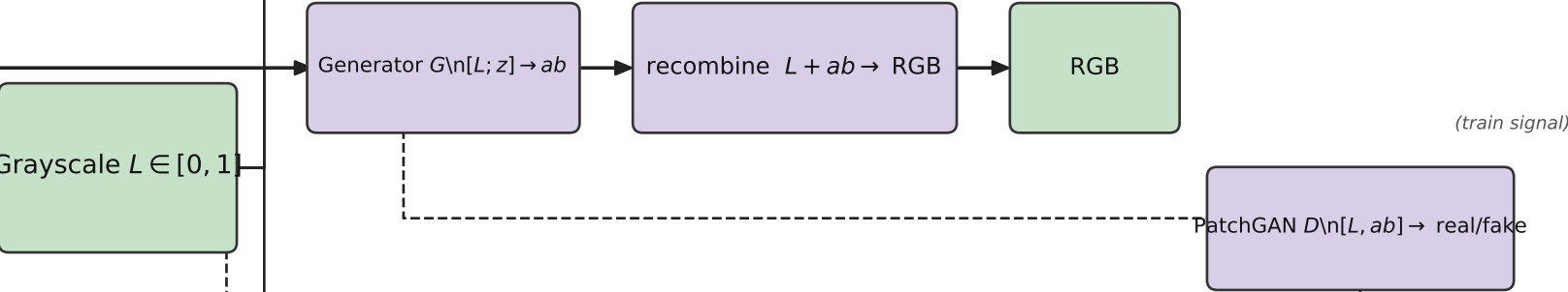
Path B — Conditional GAN
