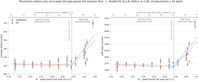
Fig. 2. Mean delay against peak link load PL under local (buffer-level) selection, PF marked. Below the floor a 3.07\times spread in PL moves delay 1.15\text{--}1.18\times (n.s.); above it a 1.20\times spread moves delay 1.71\text{--}1.85\times . [TODO: replace with E1-grid version, BL only]
