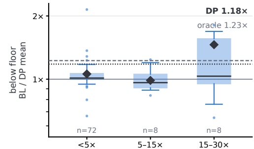
ResNet-50
