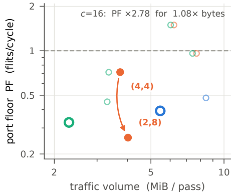
ResNet-50
