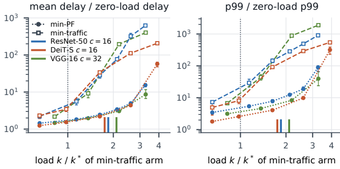
Fig. 2. Min-PF (dotted) vs. min-traffic (dashed) orientation under BL; load relative to the min-traffic arm's k^* , delay to zero load; ticks mark the min-PF arm's k^* .
