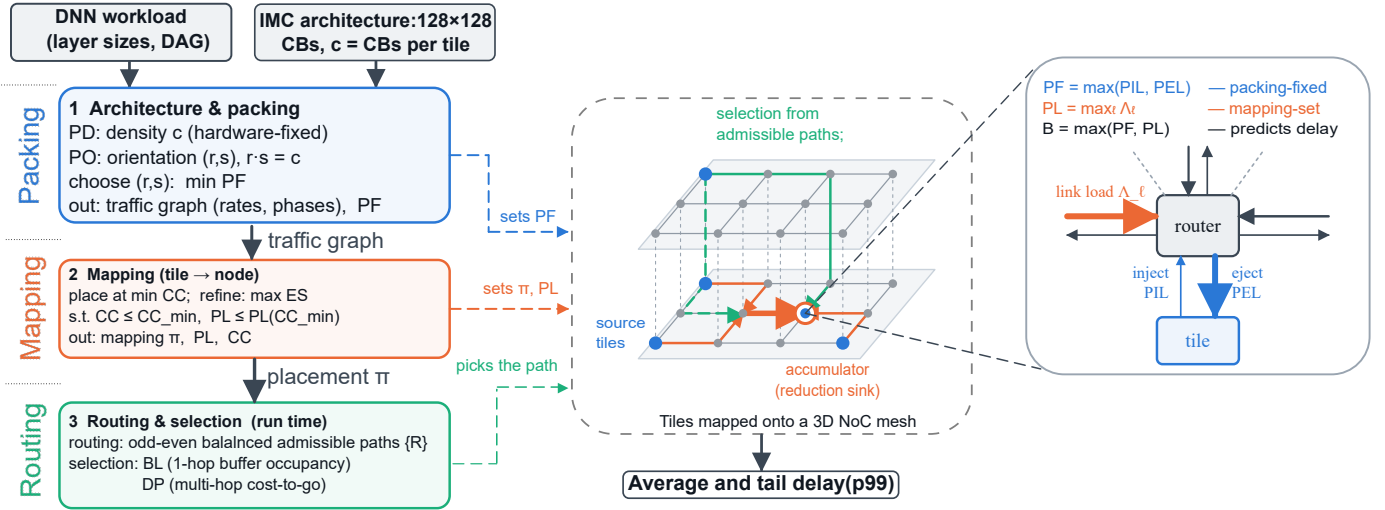
Fig. 1. The layered design flow (left), what each layer sets on the 3D NoC (center), and one node's ports and links (right).
