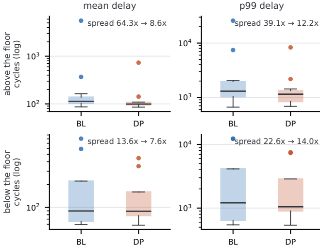
Fig. 5. BL vs. DP across placements: 12 equal-PL placements of ResNet-50 (16, 2, 8) above the floor (top), 8 of (8, 1, 8) at the knee below (bottom).
