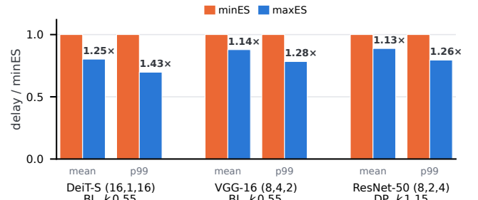
Fig. 4. maxES vs. minES per arm ( p = 0.016 on p99, three arms combined). Bars: 1/\text{mean paired ratio} ; labels: the ratio.
