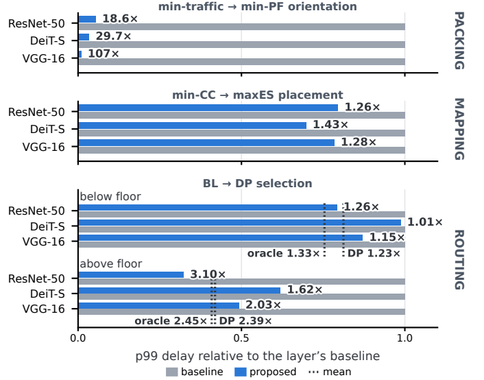
Fig. 6. p99 gain at each layer against its own baseline, per workload; routing by regime, with the pooled DP gain and the per-cell BL/DP oracle dotted.
