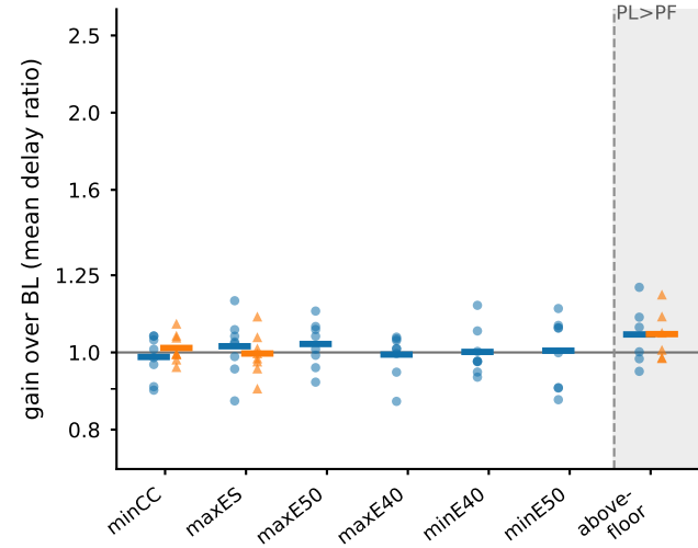
ResNet-50 (16,2,8)
