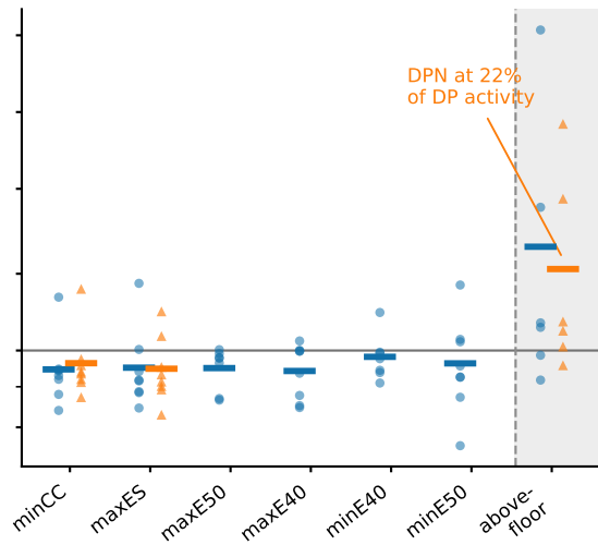
DeiT-S (16,1,16)
