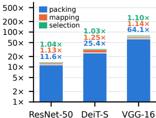
mean delay
