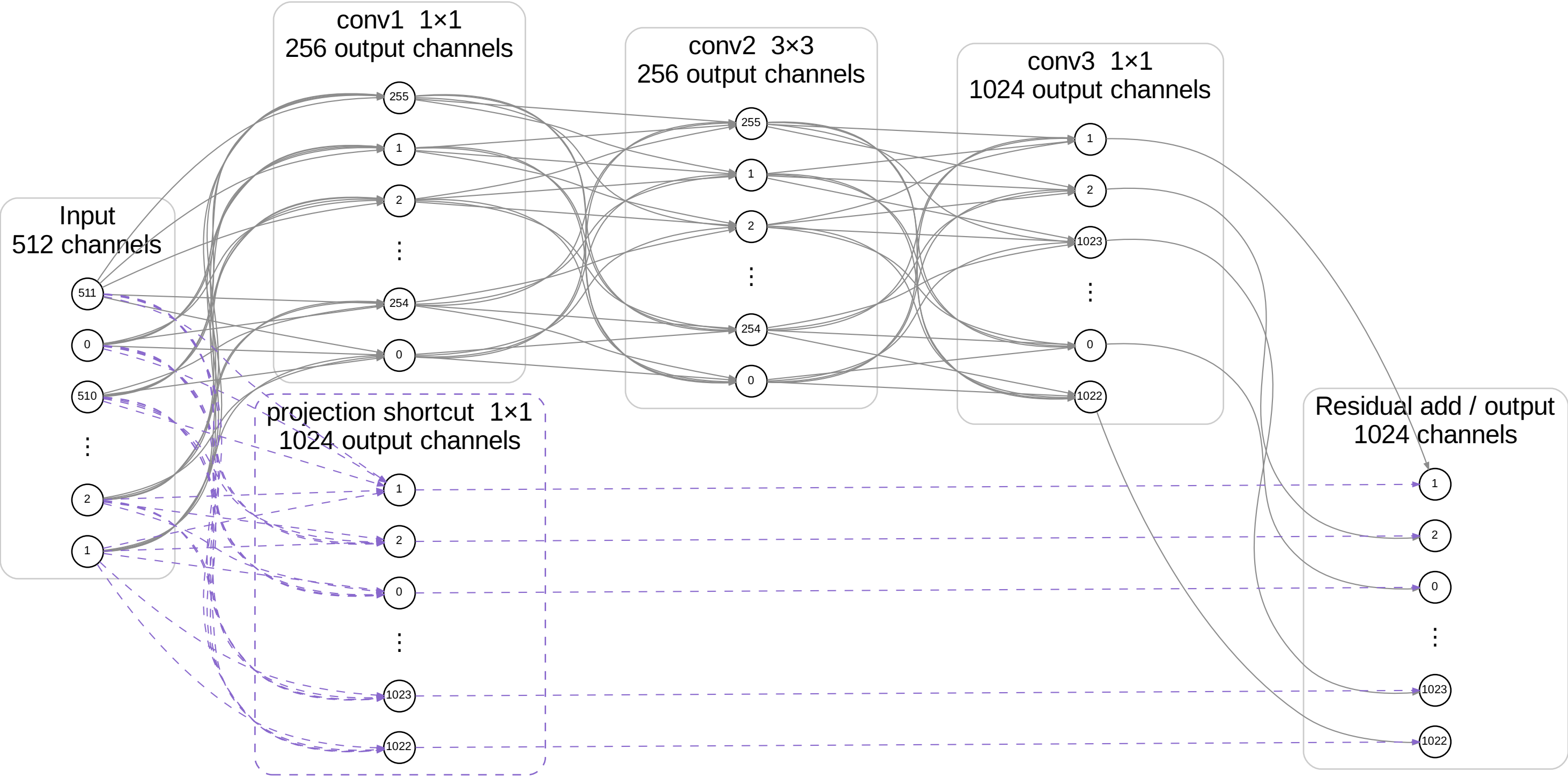
ResNet-50 stage-3 bottleneck — channel-level view
