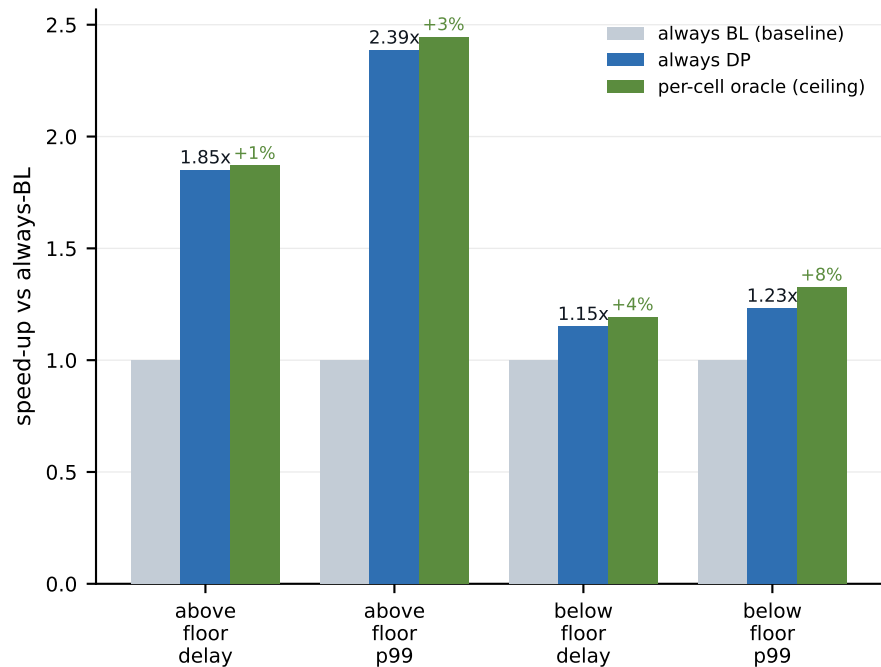
always-DP is near-optimal above, leaves 4–8% below
